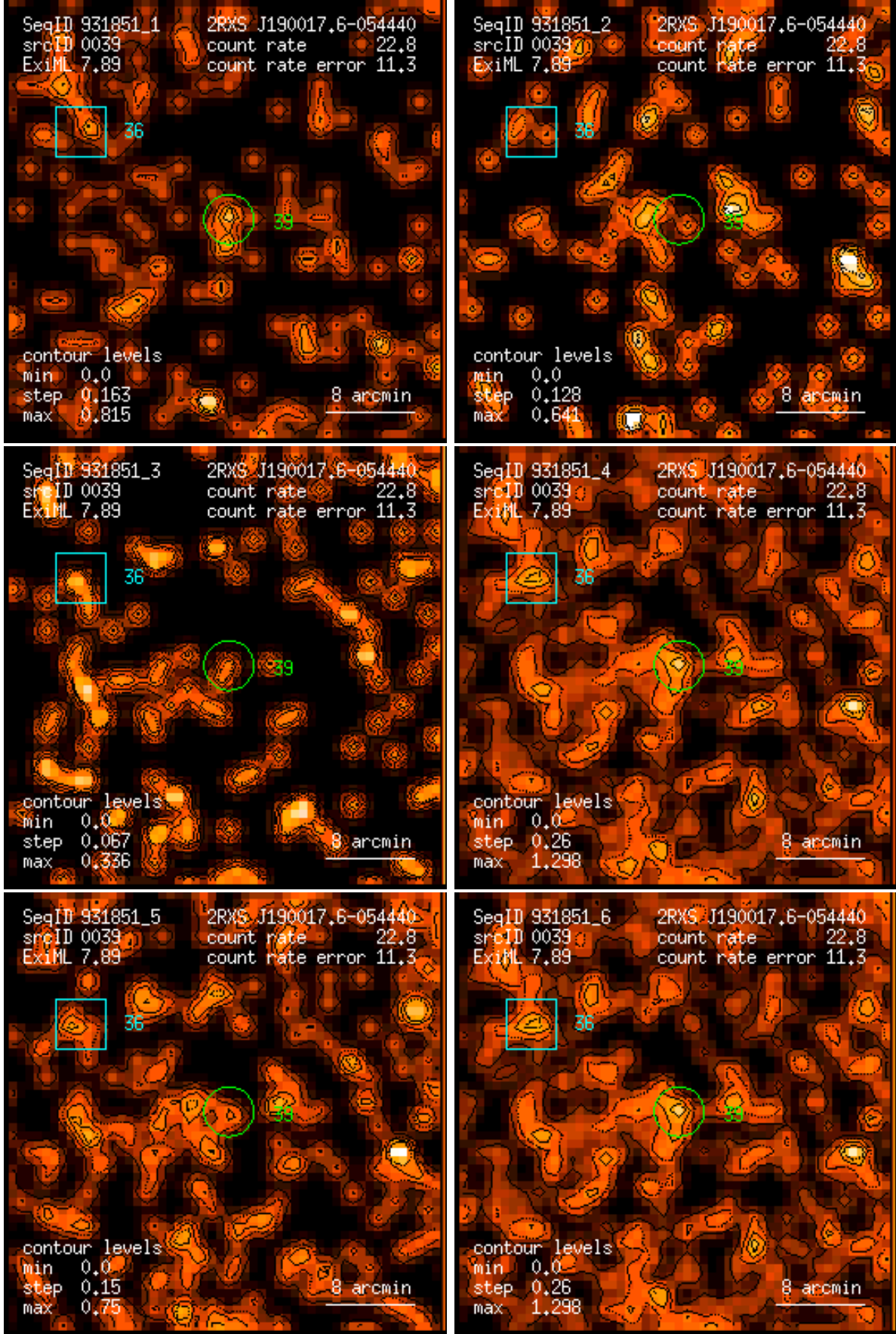
Figure 39: RASS 931851: detection 0039: band rate images, Gaussian filter: (1) PSPC channels 11 – 41, (2) 52 – 90, (3) 91 – 201, (4) 11 – 235, (5) 52 – 201, (6) 11 – 201. Broad band rates in counts/ks. Band rate contour levels in counts/ks/arcmin 2 .
