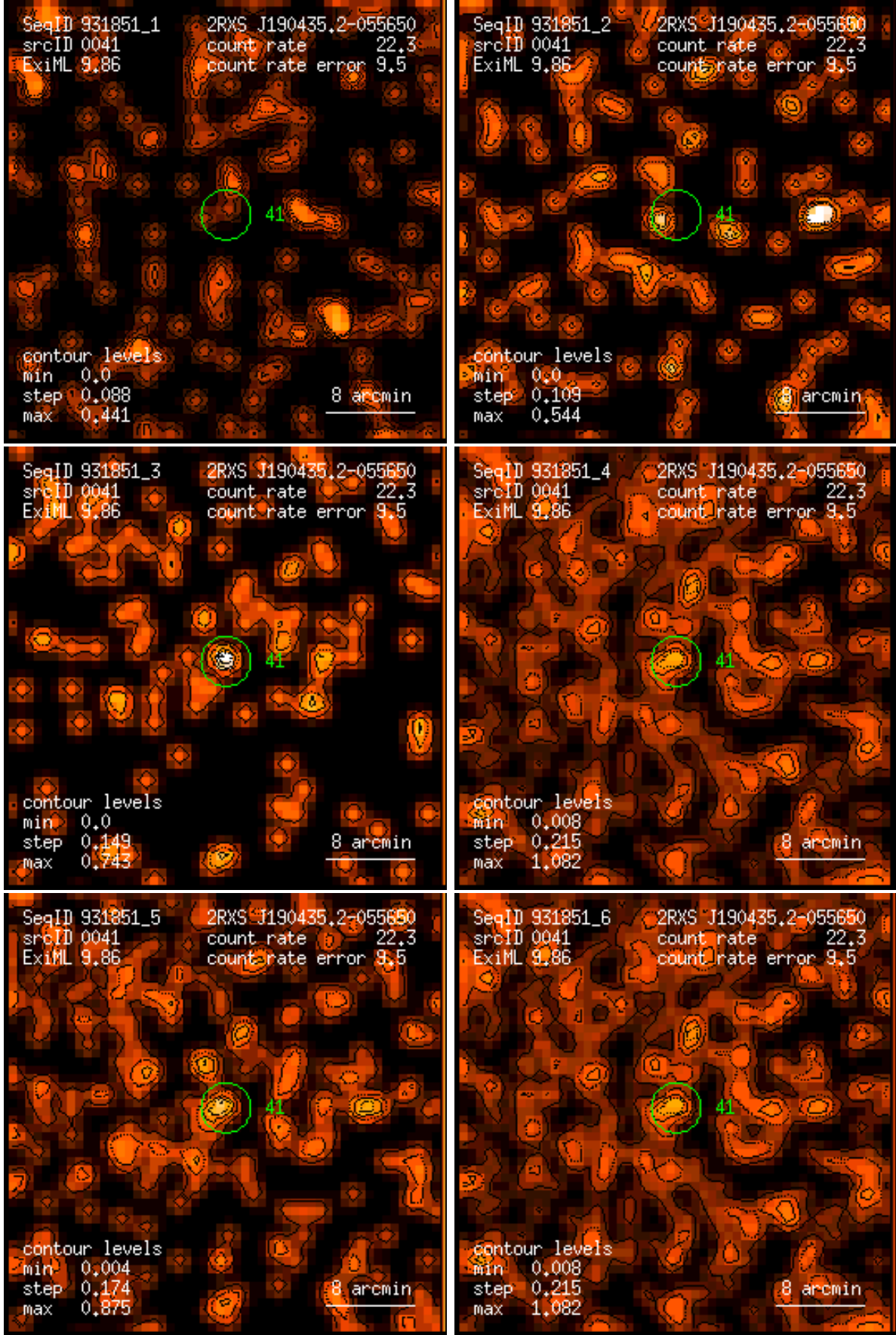
Figure 41: RASS 931851: detection 0041: band rate images, Gaussian filter: (1) PSPC channels 11 – 41, (2) 52 – 90, (3) 91 – 201, (4) 11 – 235, (5) 52 – 201, (6) 11 – 201. Broad band rates in counts/ks. Band rate contour levels in counts/ks/arcmin 2 .
