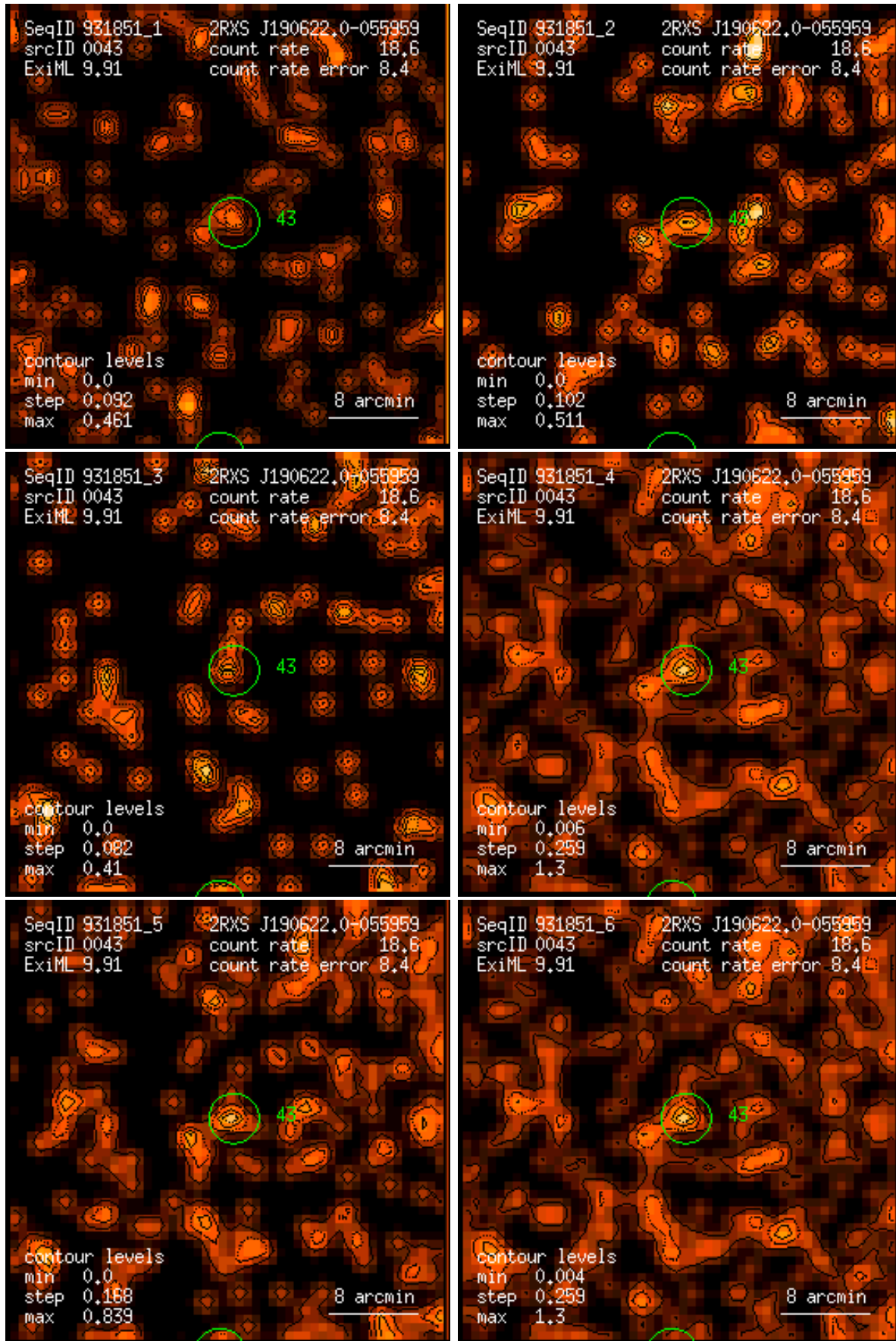
Figure 43: RASS 931851: detection 0043: band rate images, Gaussian filter: (1) PSPC channels 11 – 41, (2) 52 – 90, (3) 91 – 201, (4) 11 – 235, (5) 52 – 201, (6) 11 – 201. Broad band rates in counts/ks. Band rate contour levels in counts/ks/arcmin 2 .
