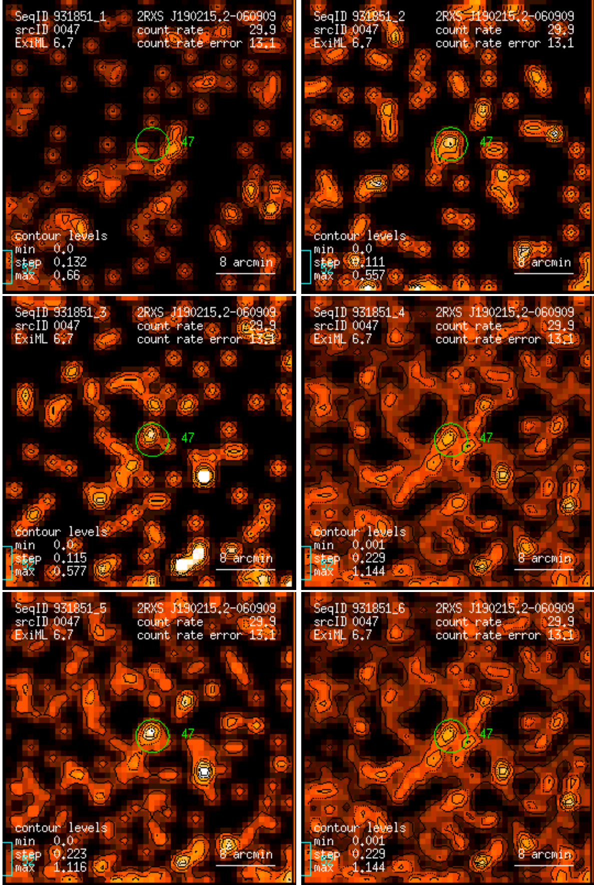
Figure 47: RASS 931851: detection 0047: band rate images, Gaussian filter: (1) PSPC channels 11 – 41, (2) 52 – 90, (3) 91 – 201, (4) 11 – 235, (5) 52 – 201, (6) 11 – 201. Broad band rates in counts/ks. Band rate contour levels in counts/ks/arcmin 2 .
