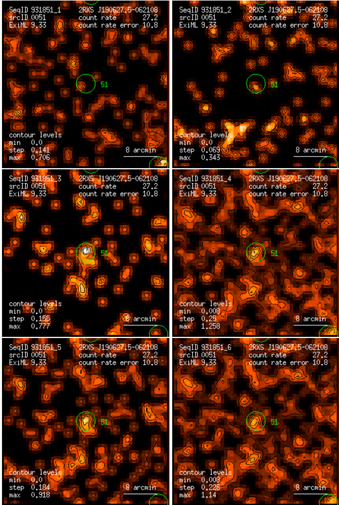
Figure 51: RASS 931851: detection 0051: band rate images, Gaussian filter: (1) PSPC channels 11 – 41, (2) 52 – 90, (3) 91 – 201, (4) 11 – 235, (5) 52 – 201, (6) 11 – 201. Broad band rates in counts/ks. Band rate contour levels in counts/ks/arcmin 2 .
