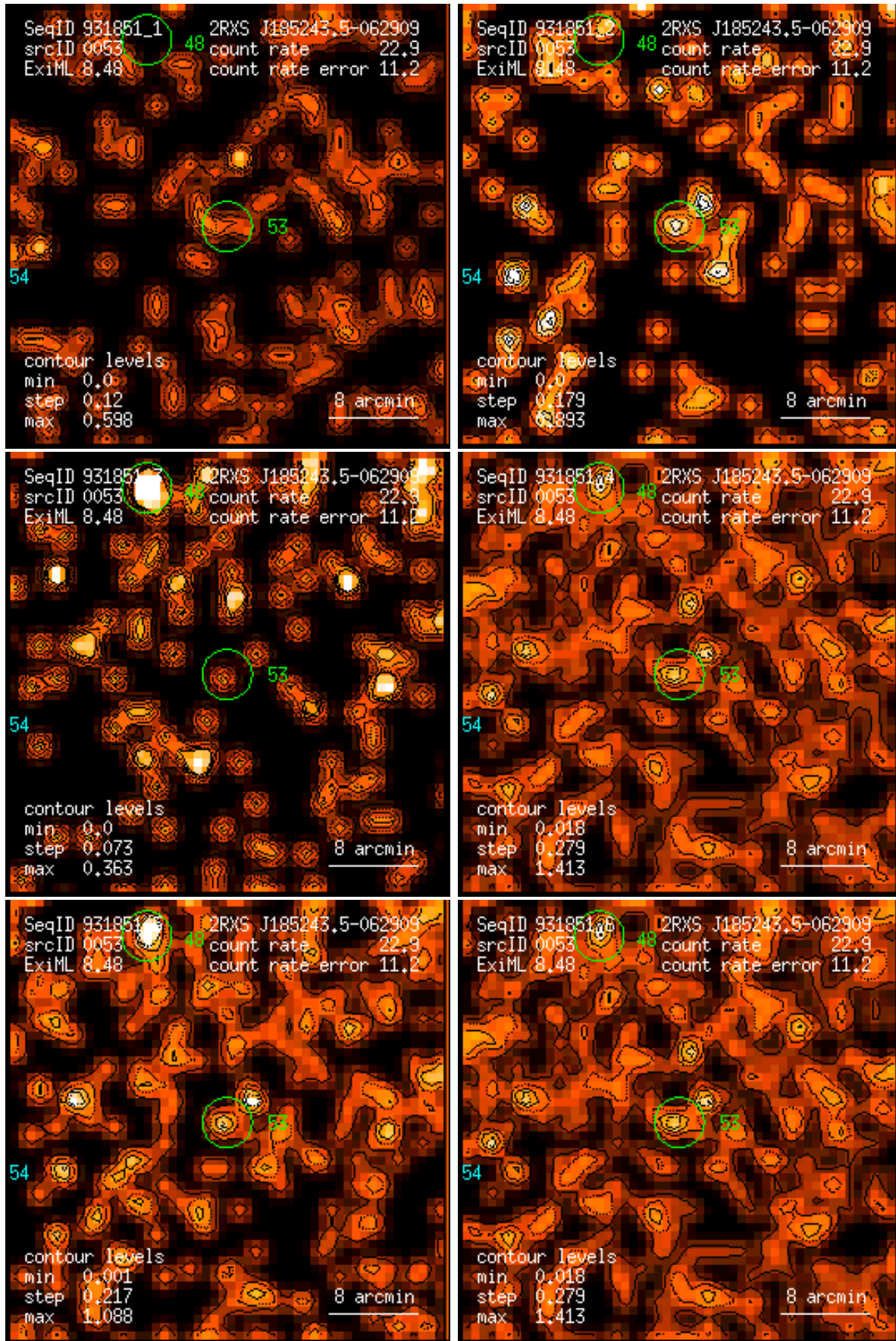
Figure 53: RASS 931851: detection 0053: band rate images, Gaussian filter: (1) PSPC channels 11 – 41, (2) 52 – 90, (3) 91 – 201, (4) 11 – 235, (5) 52 – 201, (6) 11 – 201. Broad band rates in counts/ks. Band rate contour levels in counts/ks/arcmin 2 .
