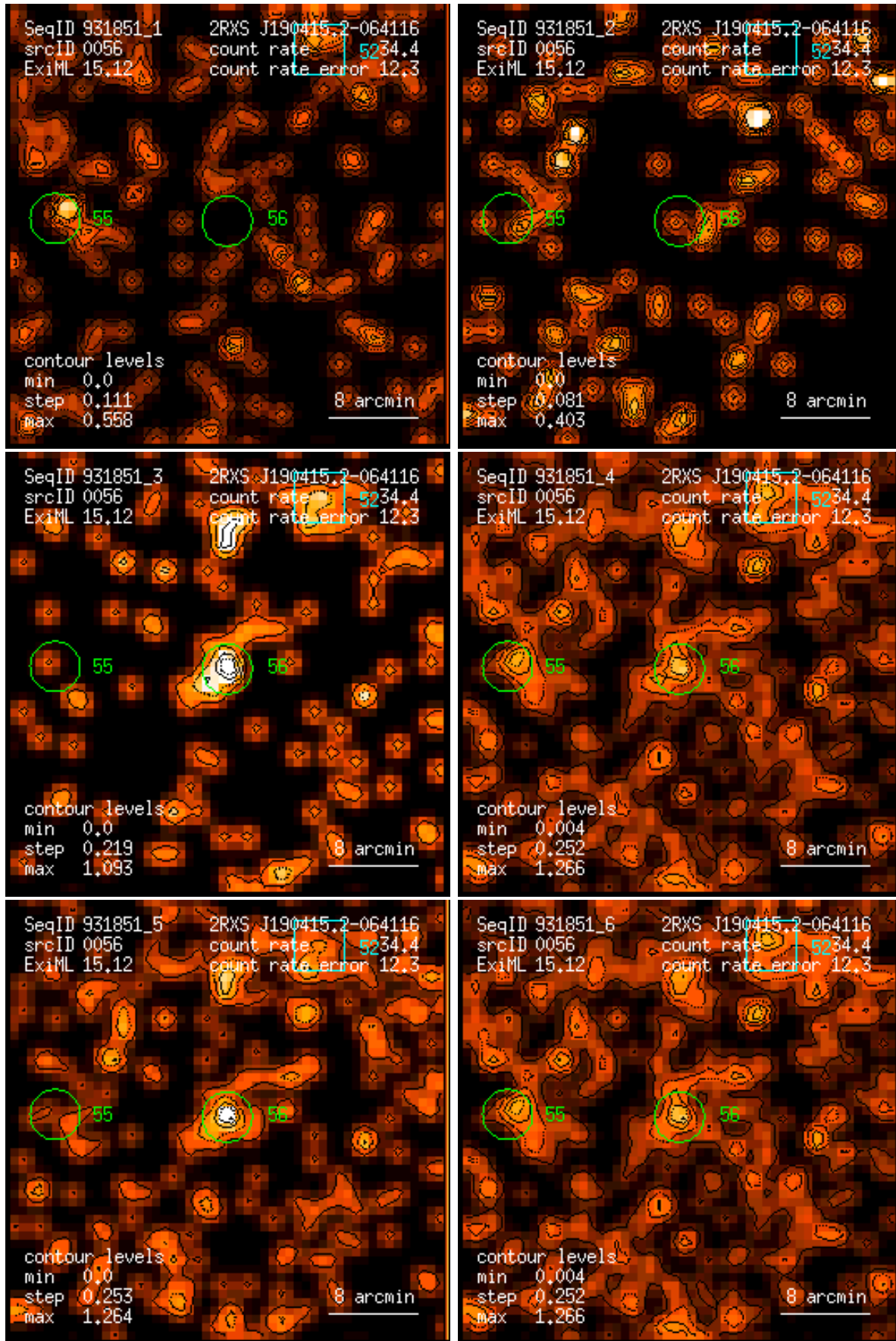
Figure 56: RASS 931851: detection 0056: band rate images, Gaussian filter: (1) PSPC channels 11 – 41, (2) 52 – 90, (3) 91 – 201, (4) 11 – 235, (5) 52 – 201, (6) 11 – 201. Broad band rates in counts/ks. Band rate contour levels in counts/ks/arcmin 2 .
