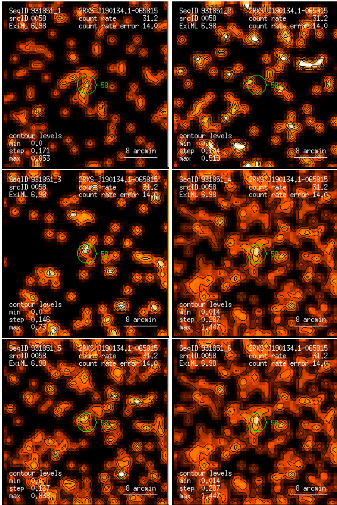
Figure 58: RASS 931851: detection 0058: band rate images, Gaussian filter: (1) PSPC channels 11 – 41, (2) 52 – 90, (3) 91 – 201, (4) 11 – 235, (5) 52 – 201, (6) 11 – 201. Broad band rates in counts/ks. Band rate contour levels in counts/ks/arcmin 2 .
