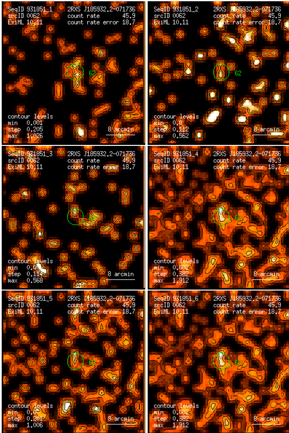
Figure 62: RASS 931851: detection 0062: band rate images, Gaussian filter: (1) PSPC channels 11 – 41, (2) 52 – 90, (3) 91 – 201, (4) 11 – 235, (5) 52 – 201, (6) 11 – 201. Broad band rates in counts/ks. Band rate contour levels in counts/ks/arcmin 2 .
