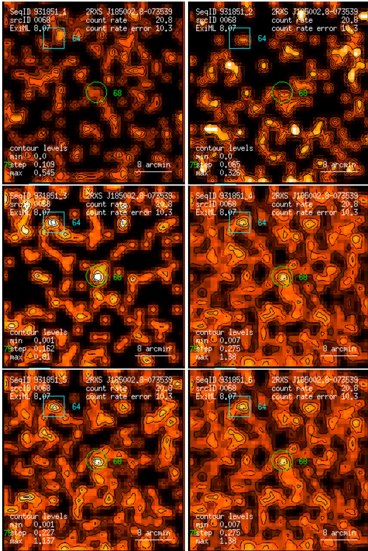
Figure 68: RASS 931851: detection 0068: band rate images, Gaussian filter: (1) PSPC channels 11 – 41, (2) 52 – 90, (3) 91 – 201, (4) 11 – 235, (5) 52 – 201, (6) 11 – 201. Broad band rates in counts/ks. Band rate contour levels in counts/ks/arcmin 2 .
