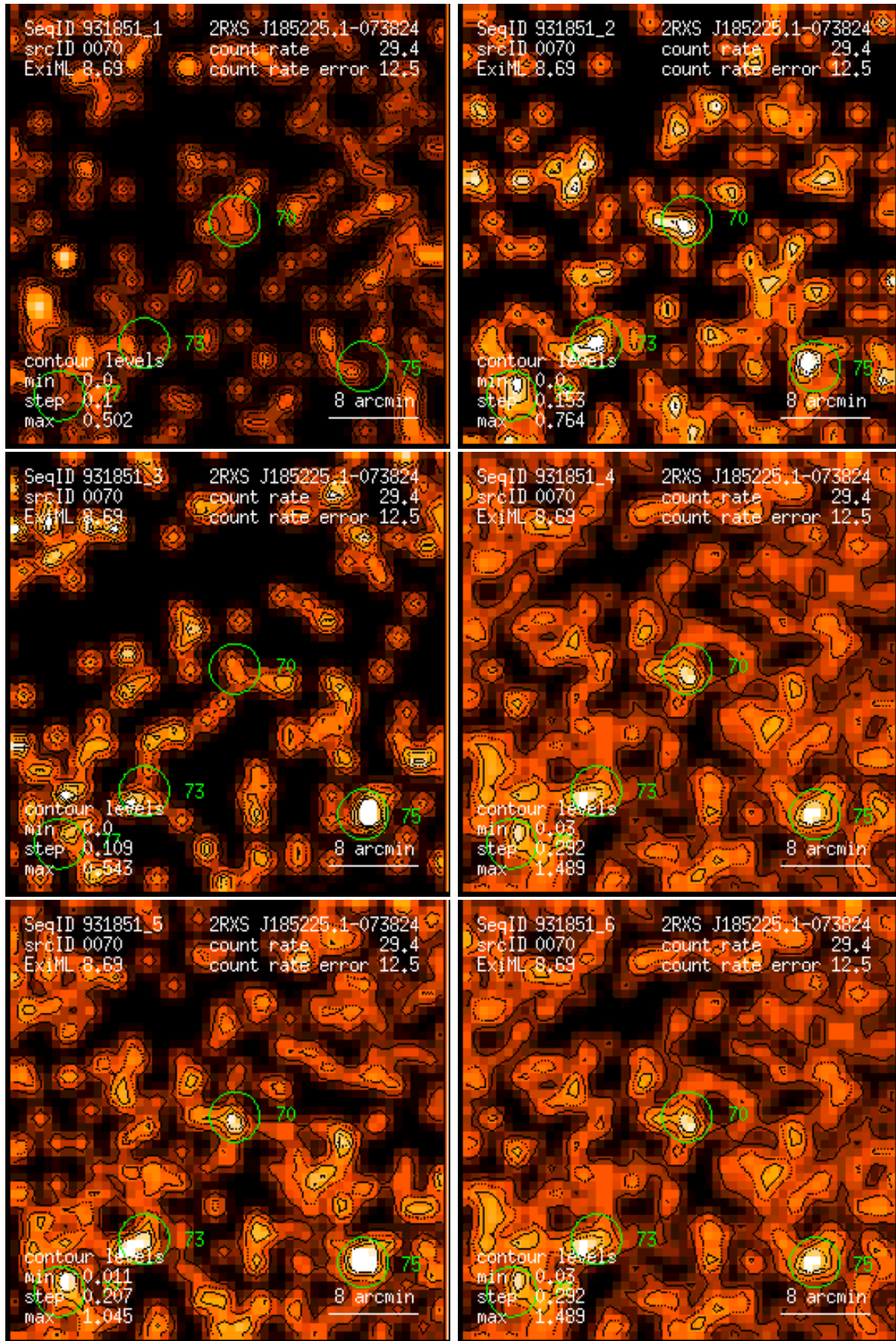
Figure 70: RASS 931851: detection 0070: band rate images, Gaussian filter: (1) PSPC channels 11 – 41, (2) 52 – 90, (3) 91 – 201, (4) 11 – 235, (5) 52 – 201, (6) 11 – 201. Broad band rates in counts/ks. Band rate contour levels in counts/ks/arcmin 2 .
