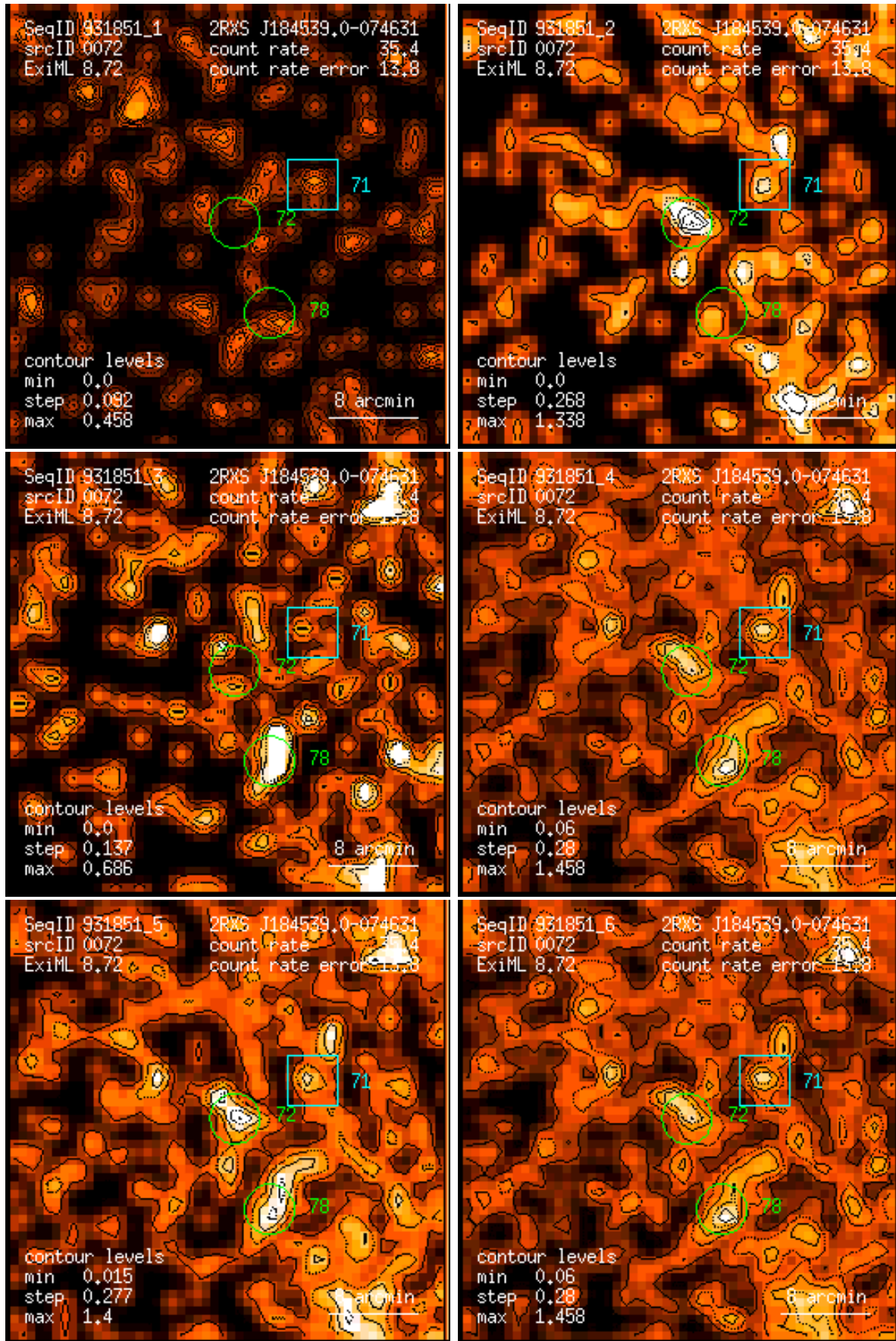
Figure 72: RASS 931851: detection 0072: band rate images, Gaussian filter: (1) PSPC channels 11 – 41, (2) 52 – 90, (3) 91 – 201, (4) 11 – 235, (5) 52 – 201, (6) 11 – 201. Broad band rates in counts/ks. Band rate contour levels in counts/ks/arcmin 2 .
