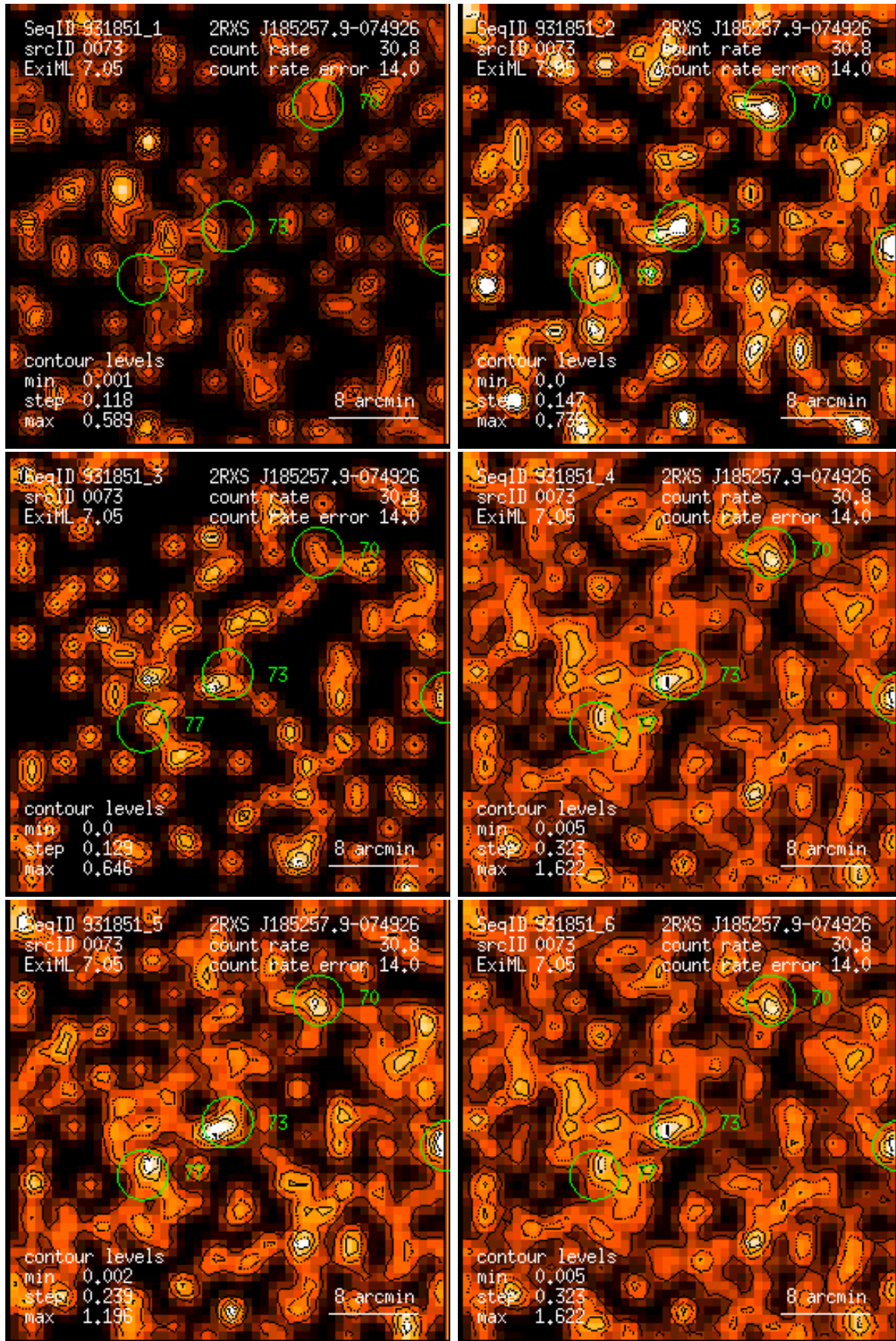
Figure 73: RASS 931851: detection 0073: band rate images, Gaussian filter: (1) PSPC channels 11 – 41, (2) 52 – 90, (3) 91 – 201, (4) 11 – 235, (5) 52 – 201, (6) 11 – 201. Broad band rates in counts/ks. Band rate contour levels in counts/ks/arcmin 2 .
