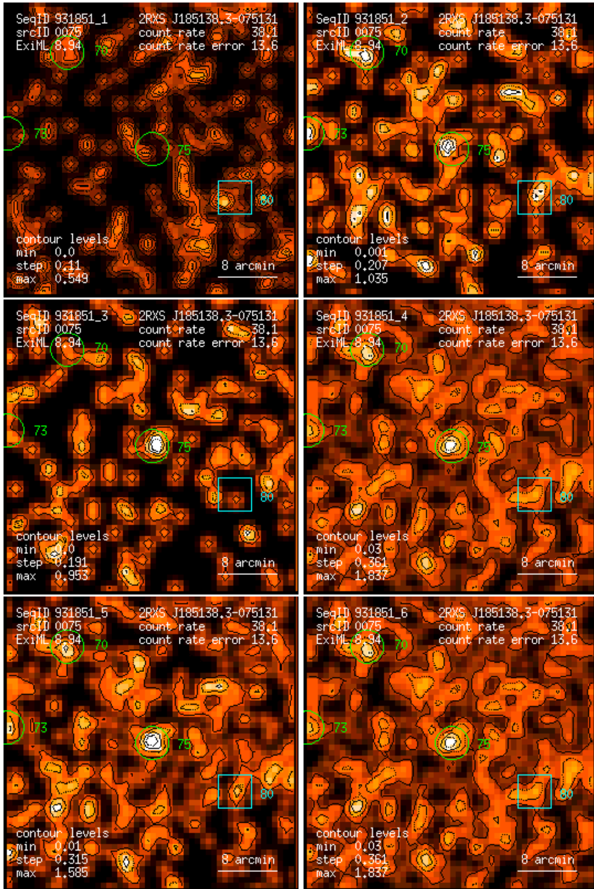
Figure 75: RASS 931851: detection 0075: band rate images, Gaussian filter: (1) PSPC channels 11 – 41, (2) 52 – 90, (3) 91 – 201, (4) 11 – 235, (5) 52 – 201, (6) 11 – 201. Broad band rates in counts/ks. Band rate contour levels in counts/ks/arcmin 2 .
