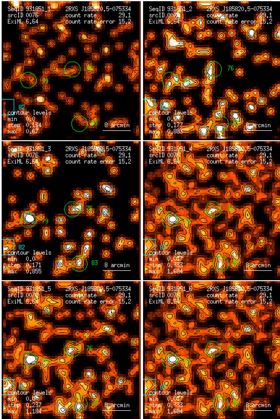
Figure 76: RASS 931851: detection 0076: band rate images, Gaussian filter: (1) PSPC channels 11 – 41, (2) 52 – 90, (3) 91 – 201, (4) 11 – 235, (5) 52 – 201, (6) 11 – 201. Broad band rates in counts/ks. Band rate contour levels in counts/ks/arcmin 2 .
