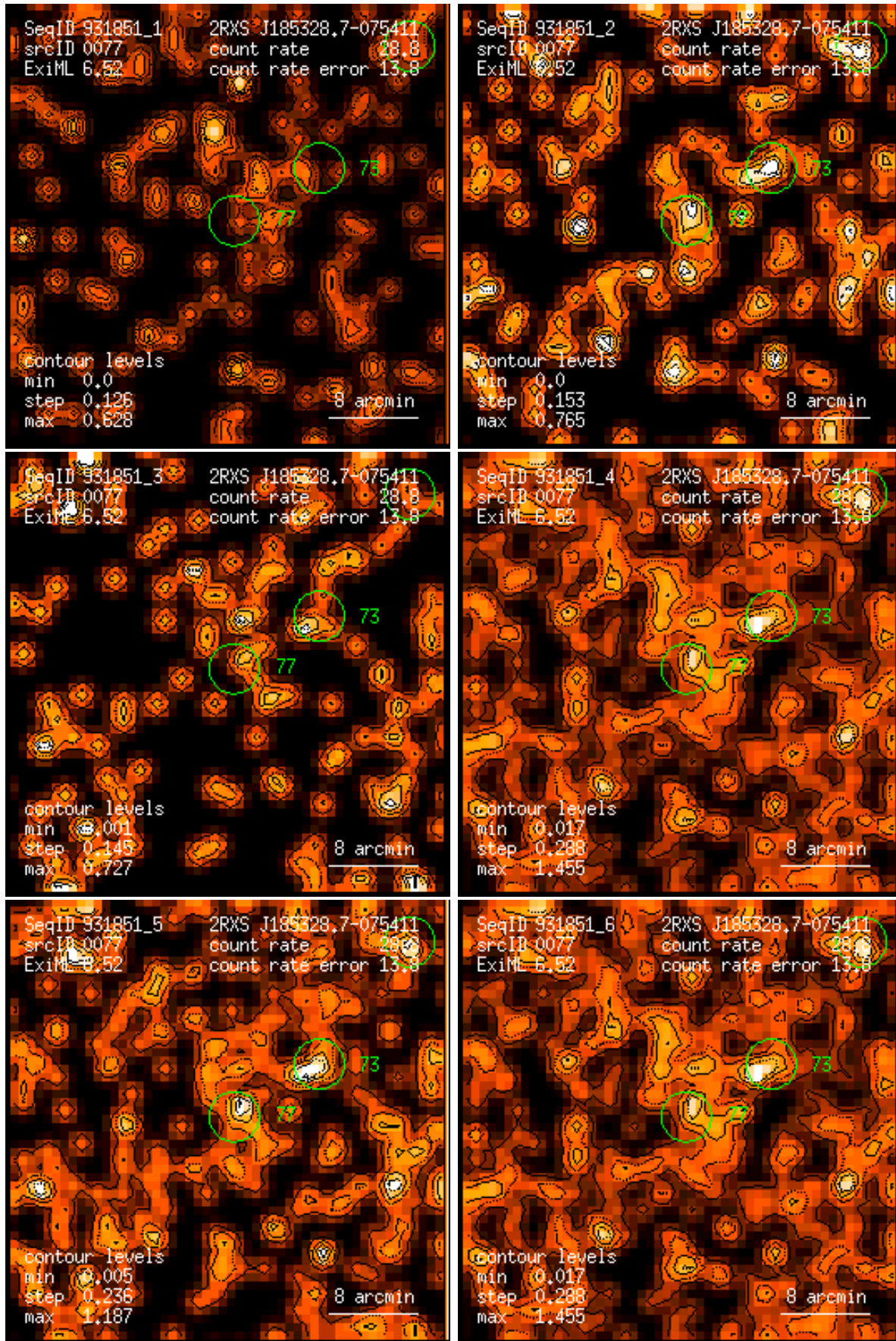
Figure 77: RASS 931851: detection 0077: band rate images, Gaussian filter: (1) PSPC channels 11 – 41, (2) 52 – 90, (3) 91 – 201, (4) 11 – 235, (5) 52 – 201, (6) 11 – 201. Broad band rates in counts/ks. Band rate contour levels in counts/ks/arcmin 2 .
