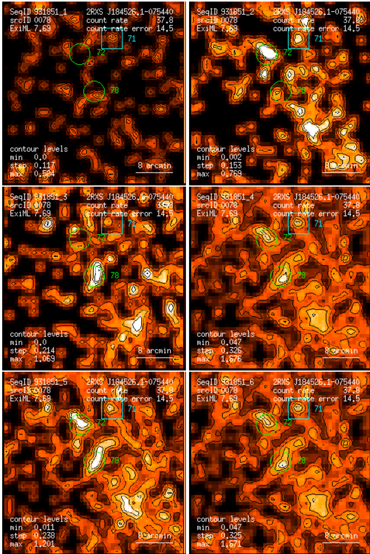
Figure 78: RASS 931851: detection 0078: band rate images, Gaussian filter: (1) PSPC channels 11 – 41, (2) 52 – 90, (3) 91 – 201, (4) 11 – 235, (5) 52 – 201, (6) 11 – 201. Broad band rates in counts/ks. Band rate contour levels in counts/ks/arcmin 2 .
