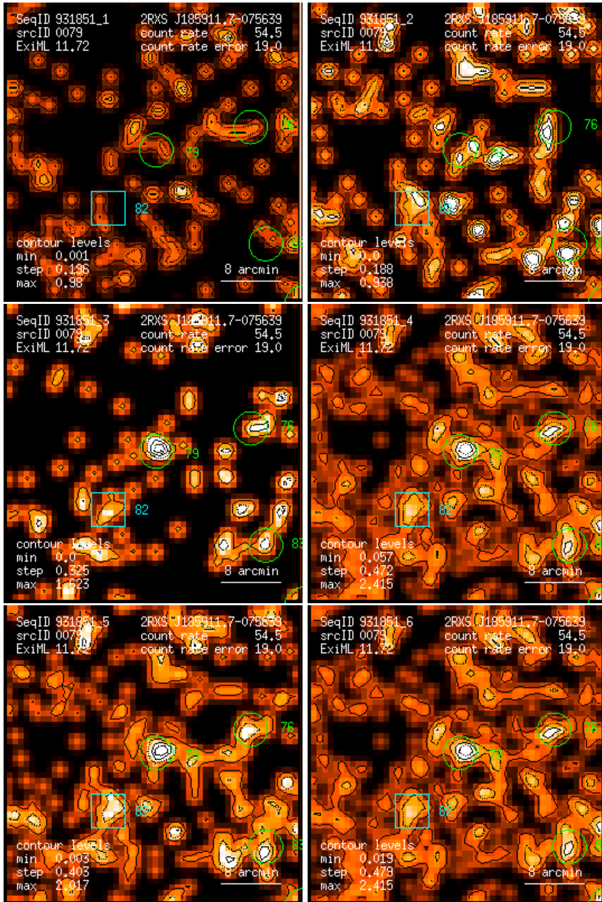
Figure 79: RASS 931851: detection 0079: band rate images, Gaussian filter: (1) PSPC channels 11 – 41, (2) 52 – 90, (3) 91 – 201, (4) 11 – 235, (5) 52 – 201, (6) 11 – 201. Broad band rates in counts/ks. Band rate contour levels in counts/ks/arcmin 2 .
