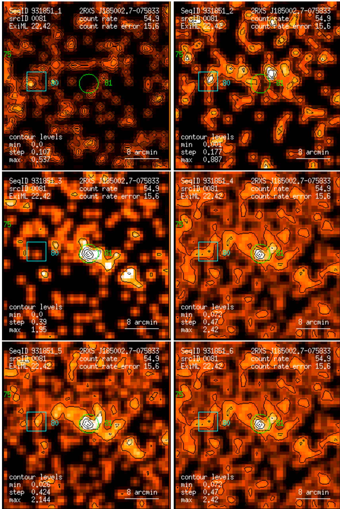
Figure 81: RASS 931851: detection 0081: band rate images, Gaussian filter: (1) PSPC channels 11 – 41, (2) 52 – 90, (3) 91 – 201, (4) 11 – 235, (5) 52 – 201, (6) 11 – 201. Broad band rates in counts/ks. Band rate contour levels in counts/ks/arcmin 2 .
