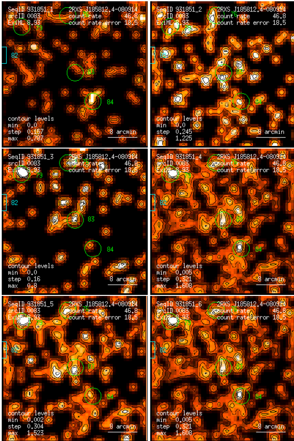
Figure 83: RASS 931851: detection 0083: band rate images, Gaussian filter: (1) PSPC channels 11 – 41, (2) 52 – 90, (3) 91 – 201, (4) 11 – 235, (5) 52 – 201, (6) 11 – 201. Broad band rates in counts/ks. Band rate contour levels in counts/ks/arcmin 2 .
