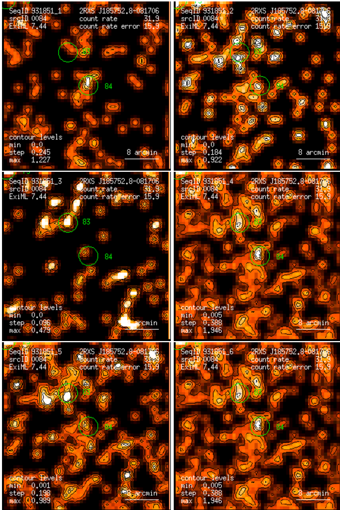
Figure 84: RASS 931851: detection 0084: band rate images, Gaussian filter: (1) PSPC channels 11 – 41, (2) 52 – 90, (3) 91 – 201, (4) 11 – 235, (5) 52 – 201, (6) 11 – 201. Broad band rates in counts/ks. Band rate contour levels in counts/ks/arcmin 2 .
