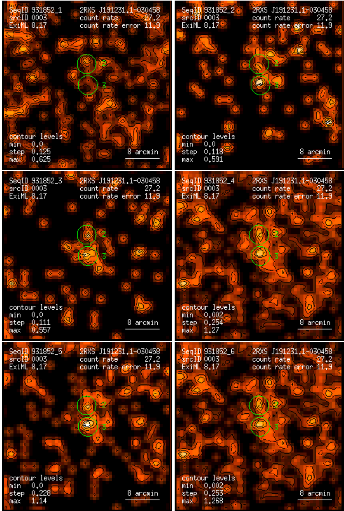
Figure 3: RASS 931852: detection 0003: band rate images, Gaussian filter: (1) PSPC channels 11 – 41, (2) 52 – 90, (3) 91 – 201, (4) 11 – 235, (5) 52 – 201, (6) 11 – 201. Broad band rates in counts/ks. Band rate contour levels in counts/ks/arcmin 2 .
