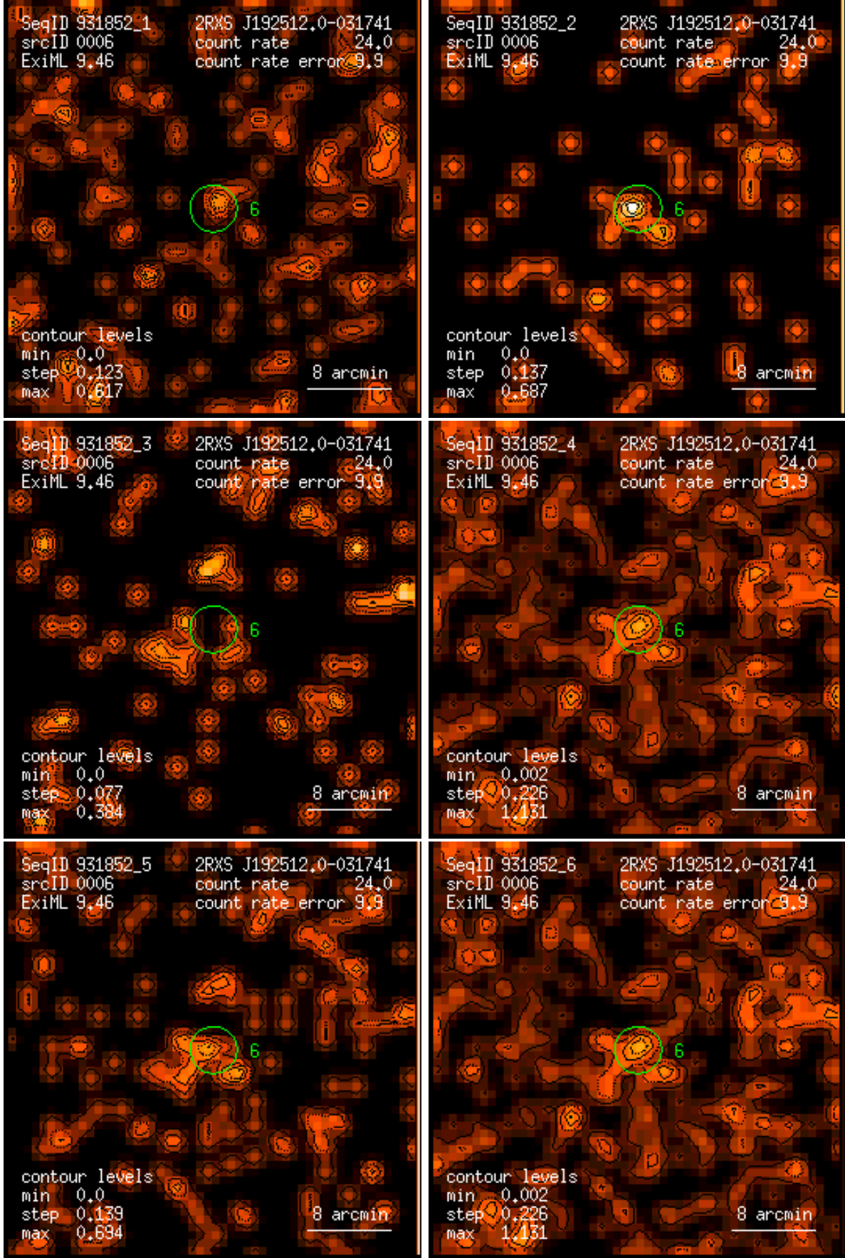
Figure 6: RASS 931852: detection 0006: band rate images, Gaussian filter: (1) PSPC channels 11 – 41, (2) 52 – 90, (3) 91 – 201, (4) 11 – 235, (5) 52 – 201, (6) 11 – 201. Broad band rates in counts/ks. Band rate contour levels in counts/ks/arcmin 2 .
