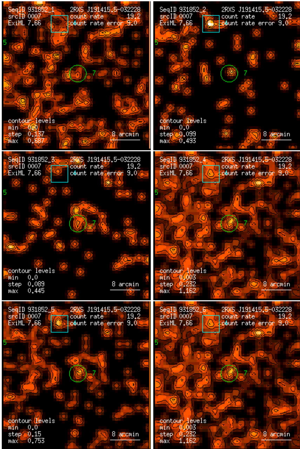
Figure 7: RASS 931852: detection 0007: band rate images, Gaussian filter: (1) PSPC channels 11 – 41, (2) 52 – 90, (3) 91 – 201, (4) 11 – 235, (5) 52 – 201, (6) 11 – 201. Broad band rates in counts/ks. Band rate contour levels in counts/ks/arcmin 2 .
