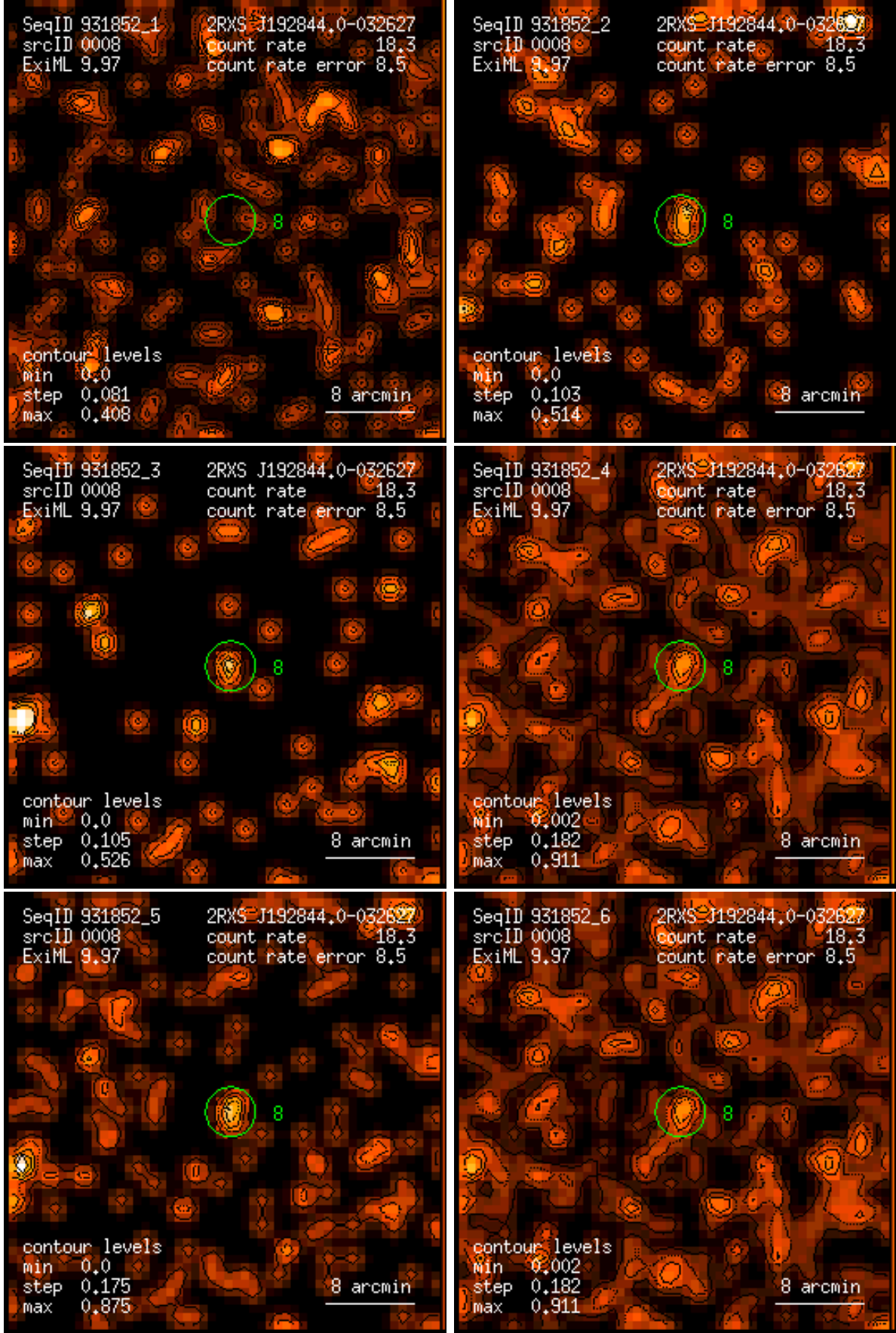
Figure 8: RASS 931852: detection 0008: band rate images, Gaussian filter: (1) PSPC channels 11 – 41, (2) 52 – 90, (3) 91 – 201, (4) 11 – 235, (5) 52 – 201, (6) 11 – 201. Broad band rates in counts/ks. Band rate contour levels in counts/ks/arcmin 2 .
