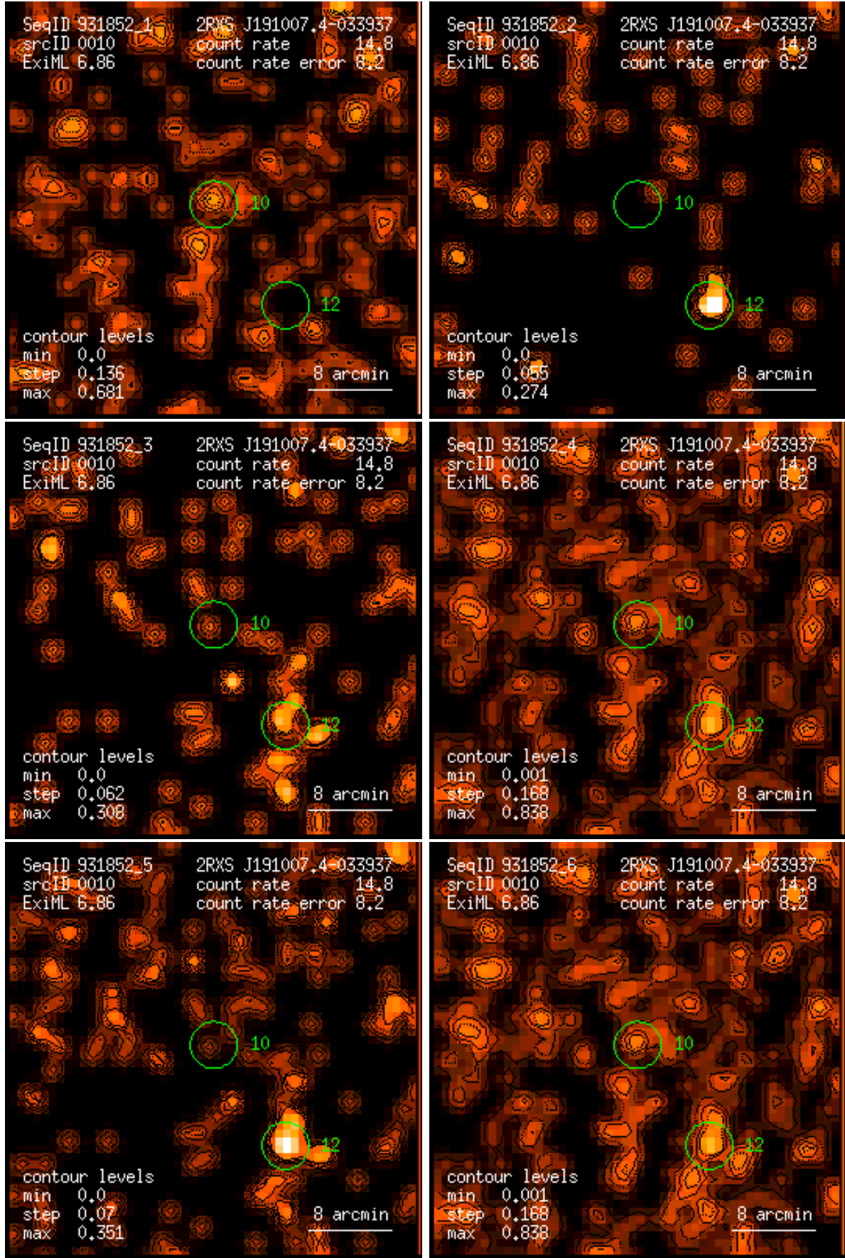
Figure 10: RASS 931852: detection 0010: band rate images, Gaussian filter: (1) PSPC channels 11 – 41, (2) 52 – 90, (3) 91 – 201, (4) 11 – 235, (5) 52 – 201, (6) 11 – 201. Broad band rates in counts/ks. Band rate contour levels in counts/ks/arcmin 2 .
