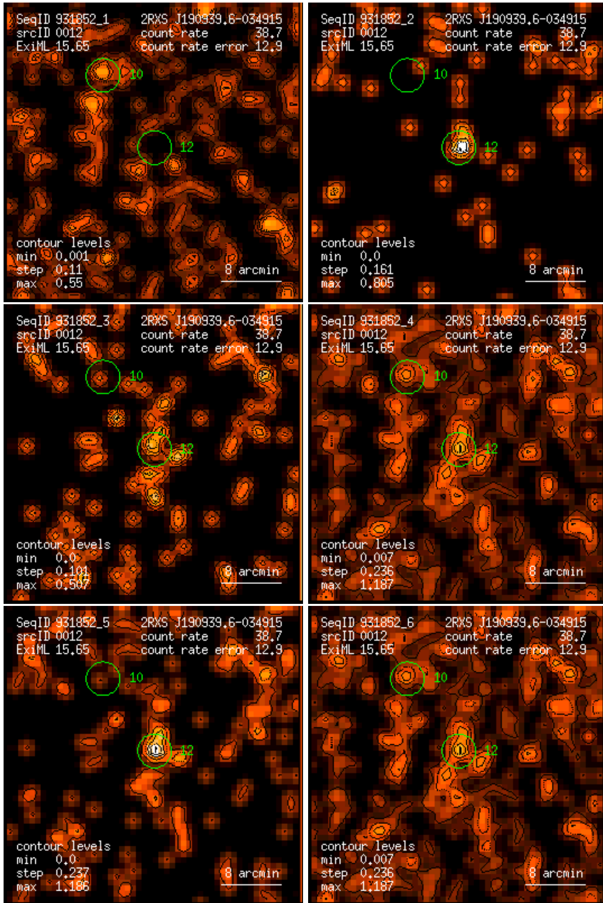
Figure 12: RASS 931852: detection 0012: band rate images, Gaussian filter: (1) PSPC channels 11 – 41, (2) 52 – 90, (3) 91 – 201, (4) 11 – 235, (5) 52 – 201, (6) 11 – 201. Broad band rates in counts/ks. Band rate contour levels in counts/ks/arcmin 2 .
