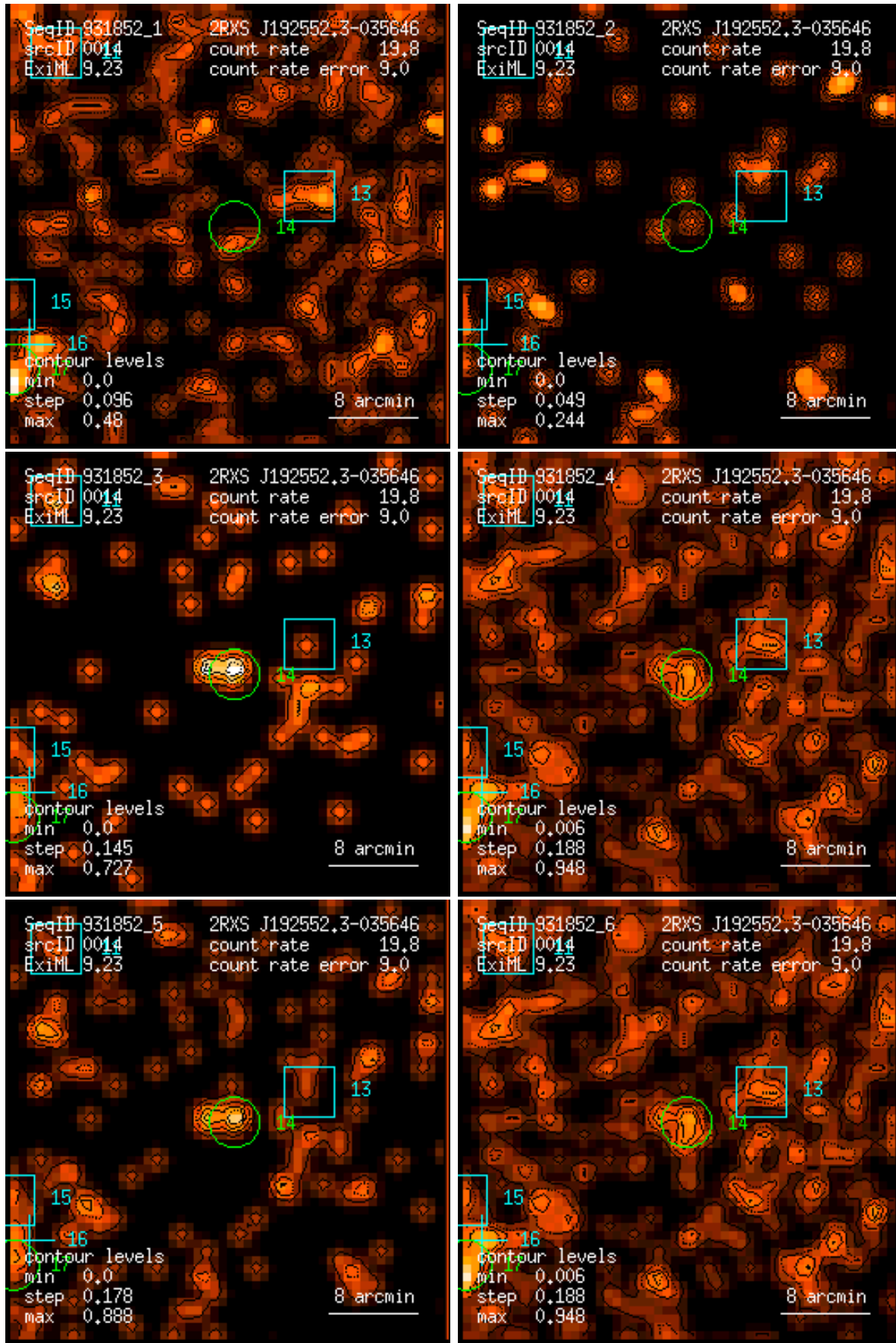
Figure 14: RASS 931852: detection 0014: band rate images, Gaussian filter: (1) PSPC channels 11 – 41, (2) 52 – 90, (3) 91 – 201, (4) 11 – 235, (5) 52 – 201, (6) 11 – 201. Broad band rates in counts/ks. Band rate contour levels in counts/ks/arcmin 2 .
