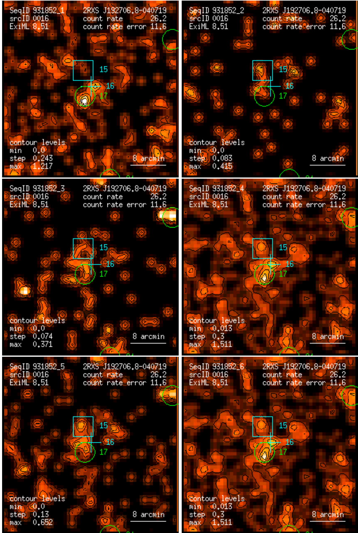
Figure 16: RASS 931852: detection 0016: band rate images, Gaussian filter: (1) PSPC channels 11 – 41, (2) 52 – 90, (3) 91 – 201, (4) 11 – 235, (5) 52 – 201, (6) 11 – 201. Broad band rates in counts/ks. Band rate contour levels in counts/ks/arcmin 2 .
