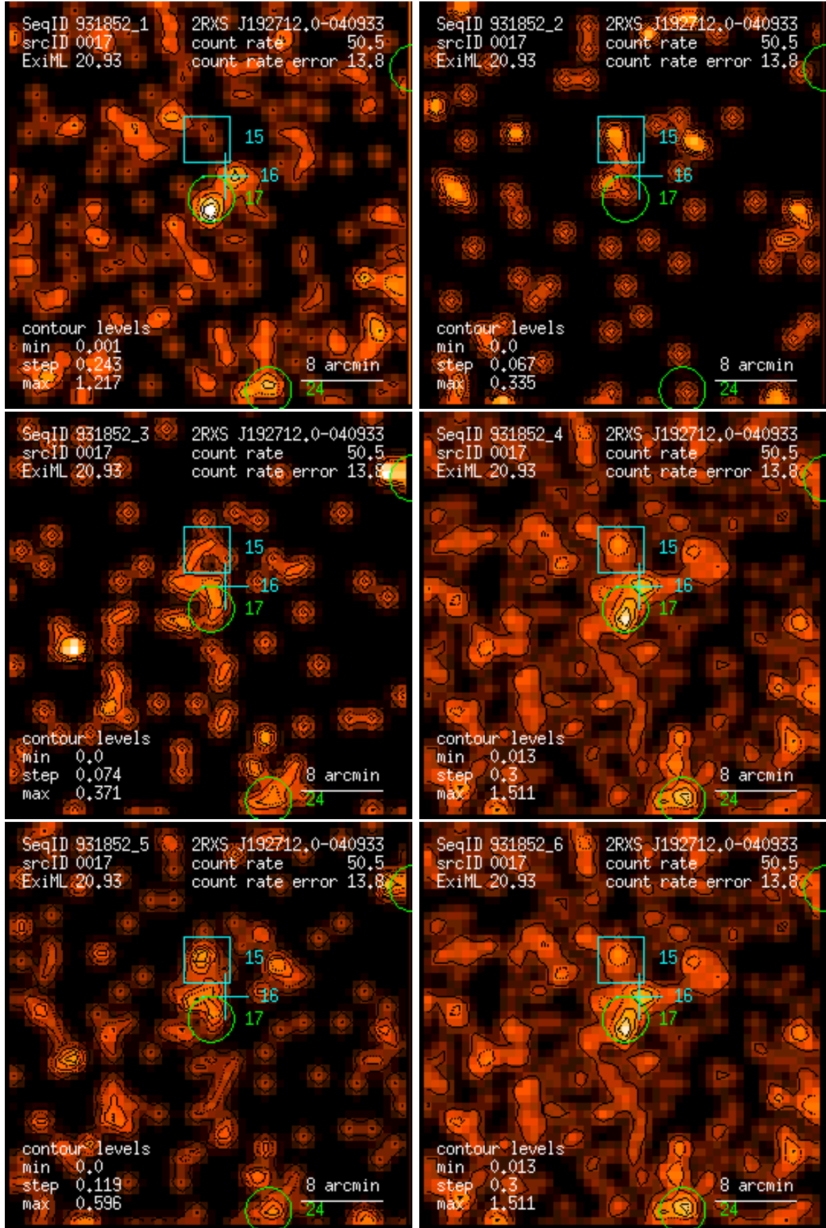
Figure 17: RASS 931852: detection 0017: band rate images, Gaussian filter: (1) PSPC channels 11 – 41, (2) 52 – 90, (3) 91 – 201, (4) 11 – 235, (5) 52 – 201, (6) 11 – 201. Broad band rates in counts/ks. Band rate contour levels in counts/ks/arcmin 2 .
