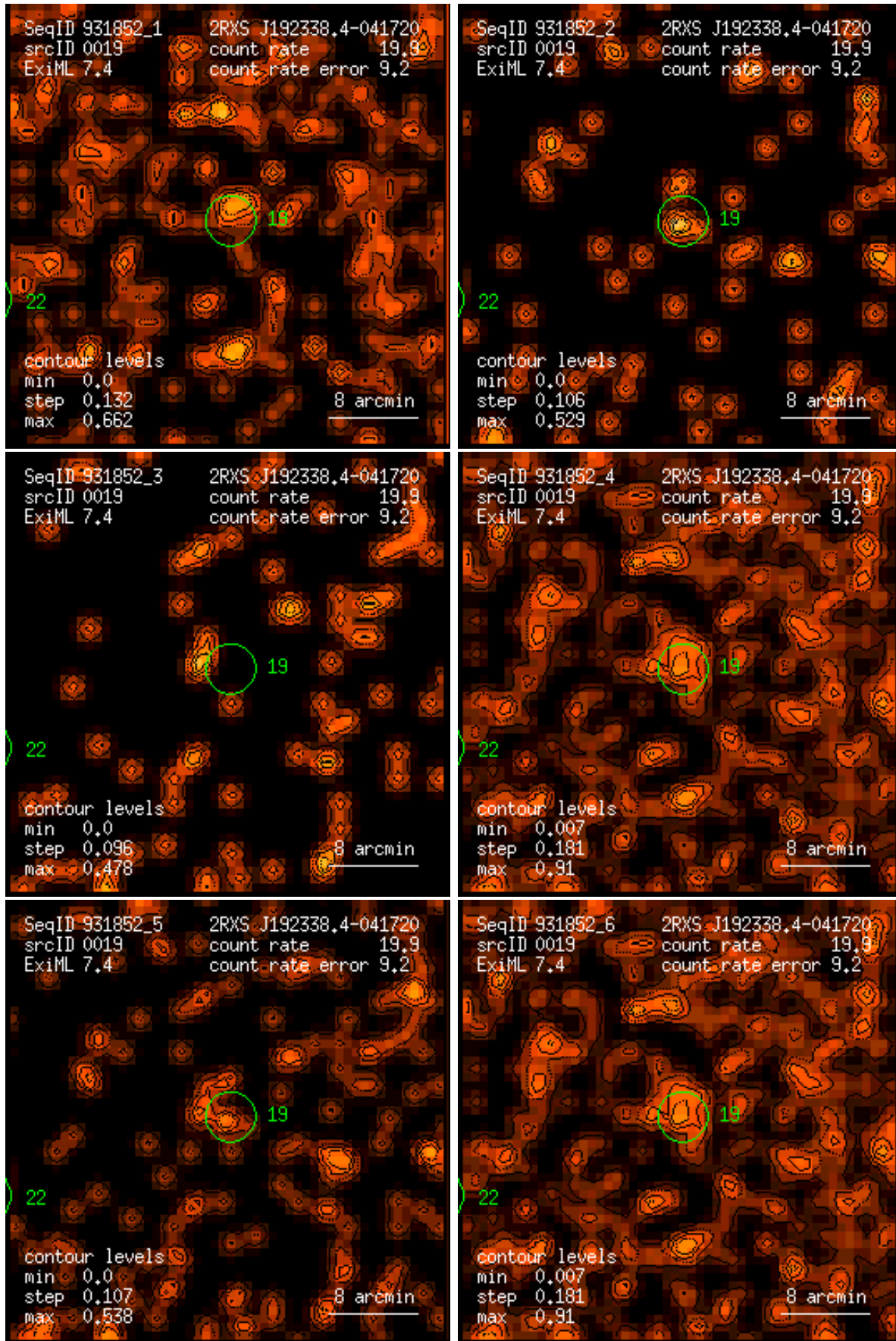
Figure 19: RASS 931852: detection 0019: band rate images, Gaussian filter: (1) PSPC channels 11 – 41, (2) 52 – 90, (3) 91 – 201, (4) 11 – 235, (5) 52 – 201, (6) 11 – 201. Broad band rates in counts/ks. Band rate contour levels in counts/ks/arcmin 2 .
