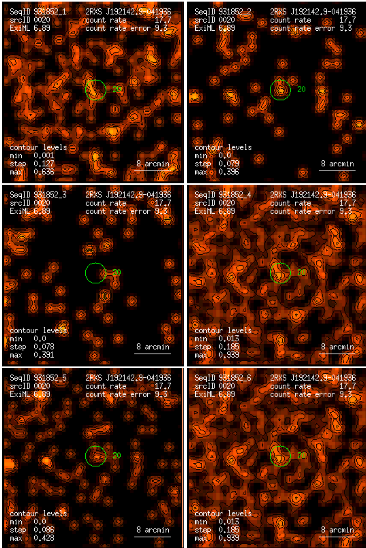
Figure 20: RASS 931852: detection 0020: band rate images, Gaussian filter: (1) PSPC channels 11 – 41, (2) 52 – 90, (3) 91 – 201, (4) 11 – 235, (5) 52 – 201, (6) 11 – 201. Broad band rates in counts/ks. Band rate contour levels in counts/ks/arcmin 2 .
