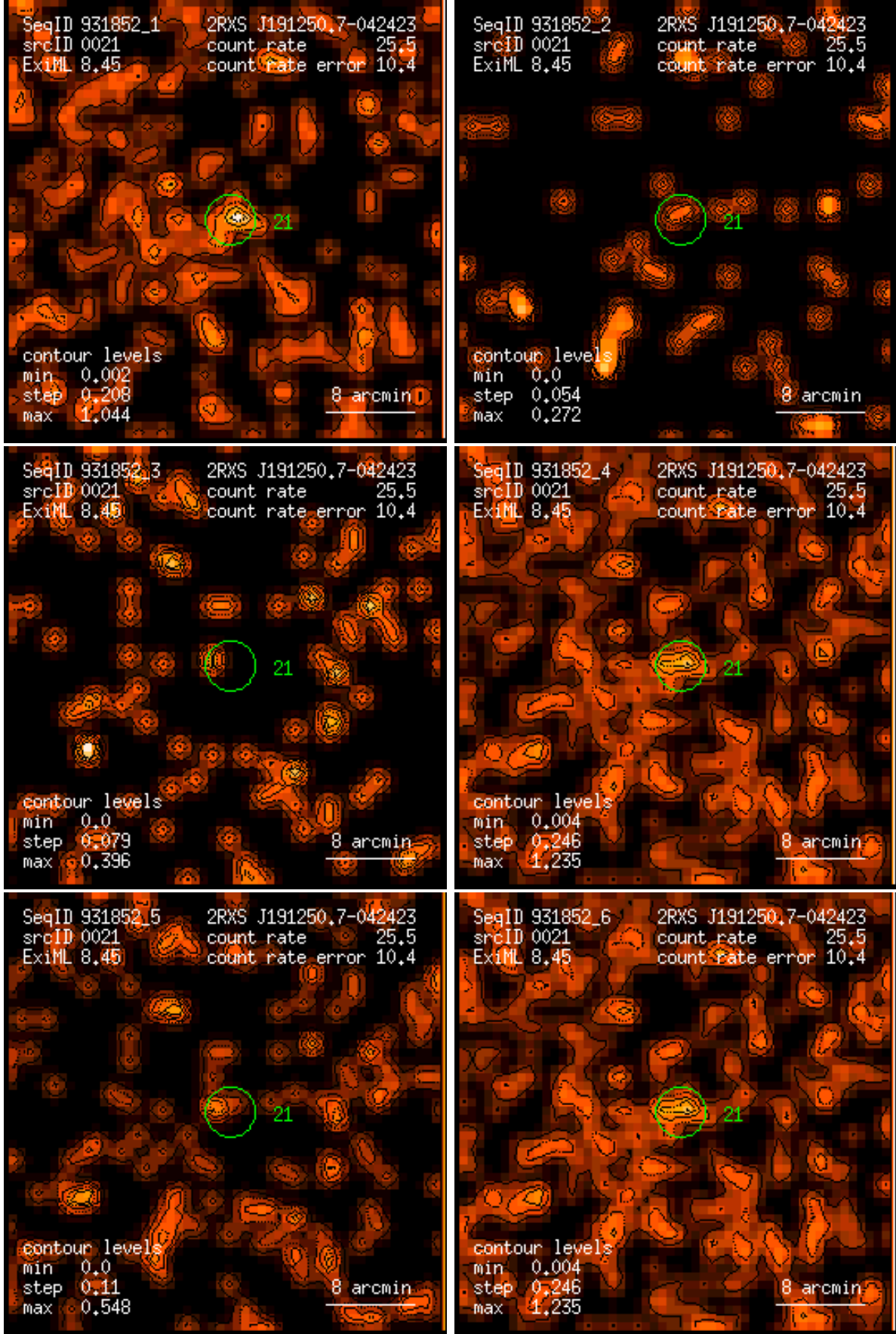
Figure 21: RASS 931852: detection 0021: band rate images, Gaussian filter: (1) PSPC channels 11 – 41, (2) 52 – 90, (3) 91 – 201, (4) 11 – 235, (5) 52 – 201, (6) 11 – 201. Broad band rates in counts/ks. Band rate contour levels in counts/ks/arcmin 2 .
