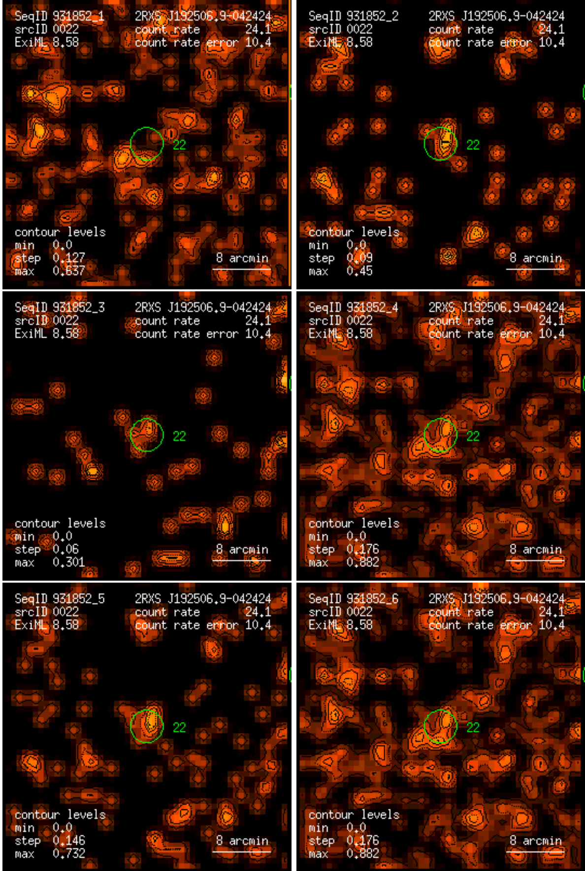
Figure 22: RASS 931852: detection 0022: band rate images, Gaussian filter: (1) PSPC channels 11 – 41, (2) 52 – 90, (3) 91 – 201, (4) 11 – 235, (5) 52 – 201, (6) 11 – 201. Broad band rates in counts/ks. Band rate contour levels in counts/ks/arcmin 2 .
