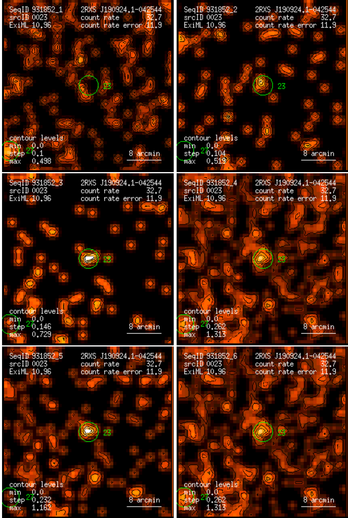
Figure 23: RASS 931852: detection 0023: band rate images, Gaussian filter: (1) PSPC channels 11 – 41, (2) 52 – 90, (3) 91 – 201, (4) 11 – 235, (5) 52 – 201, (6) 11 – 201. Broad band rates in counts/ks. Band rate contour levels in counts/ks/arcmin 2 .
