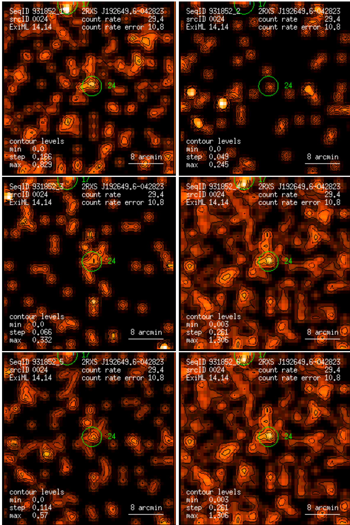
Figure 24: RASS 931852: detection 0024: band rate images, Gaussian filter: (1) PSPC channels 11 – 41, (2) 52 – 90, (3) 91 – 201, (4) 11 – 235, (5) 52 – 201, (6) 11 – 201. Broad band rates in counts/ks. Band rate contour levels in counts/ks/arcmin 2 .
