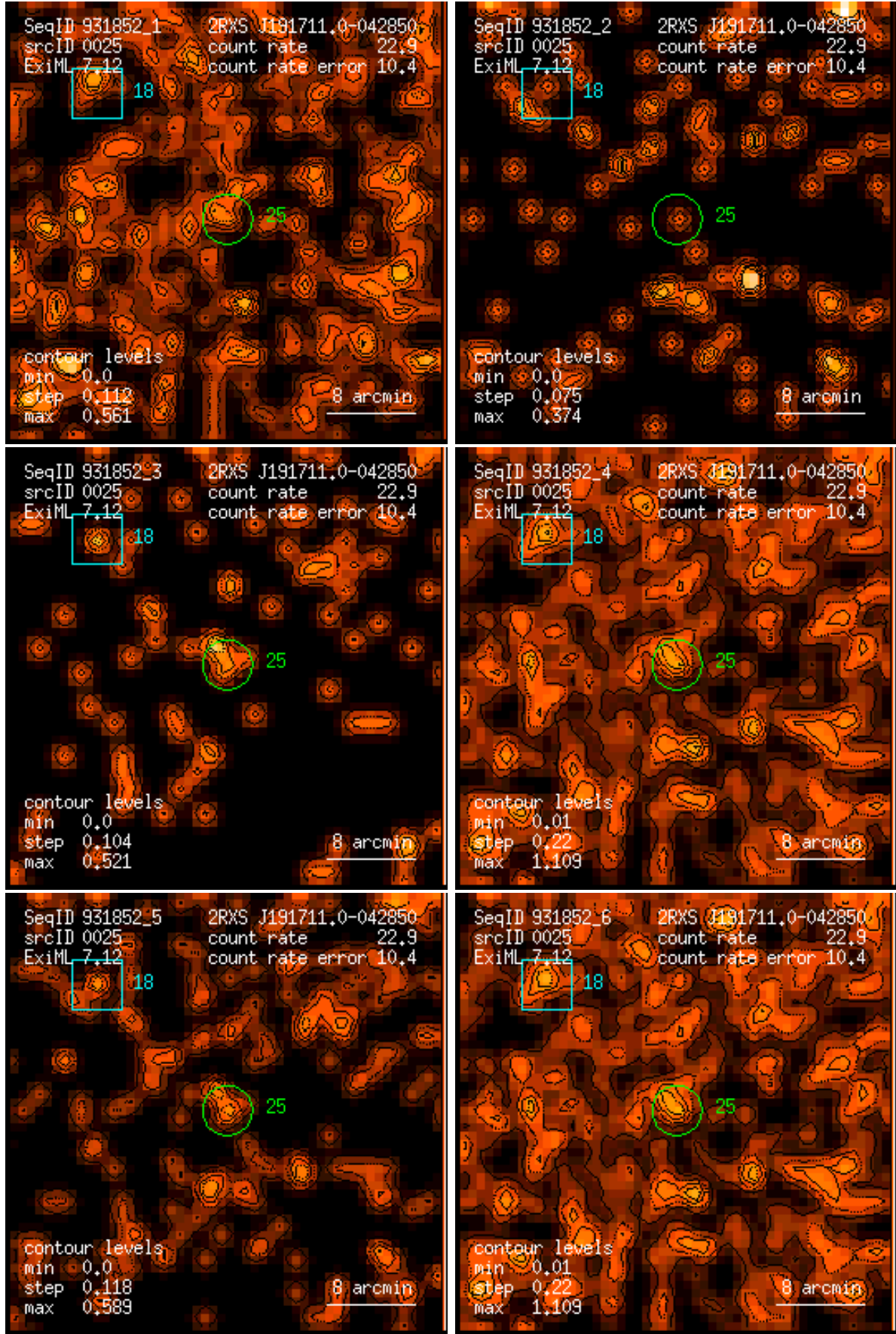
Figure 25: RASS 931852: detection 0025: band rate images, Gaussian filter: (1) PSPC channels 11 – 41, (2) 52 – 90, (3) 91 – 201, (4) 11 – 235, (5) 52 – 201, (6) 11 – 201. Broad band rates in counts/ks. Band rate contour levels in counts/ks/arcmin 2 .
