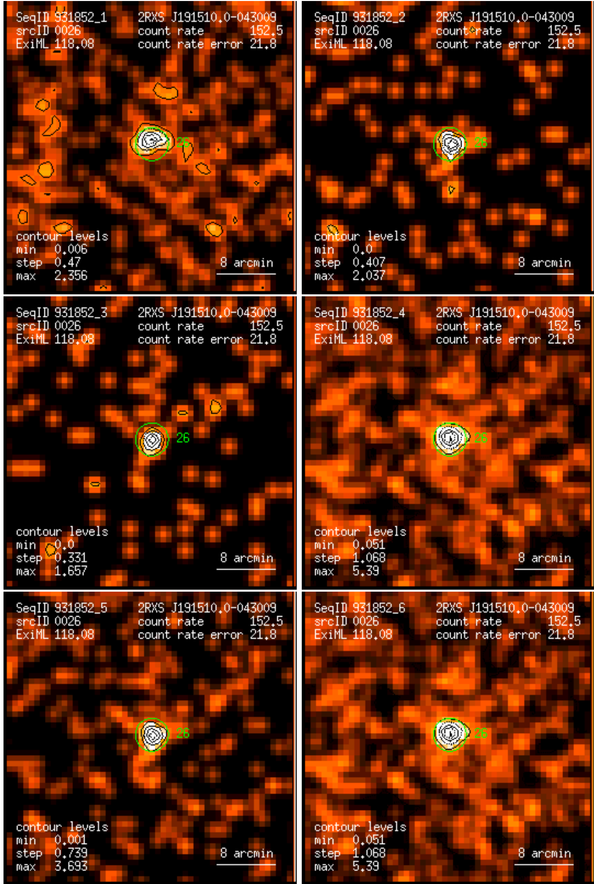
Figure 26: RASS 931852: detection 0026: band rate images, Gaussian filter: (1) PSPC channels 11 – 41, (2) 52 – 90, (3) 91 – 201, (4) 11 – 235, (5) 52 – 201, (6) 11 – 201. Broad band rates in counts/ks. Band rate contour levels in counts/ks/arcmin 2 .
