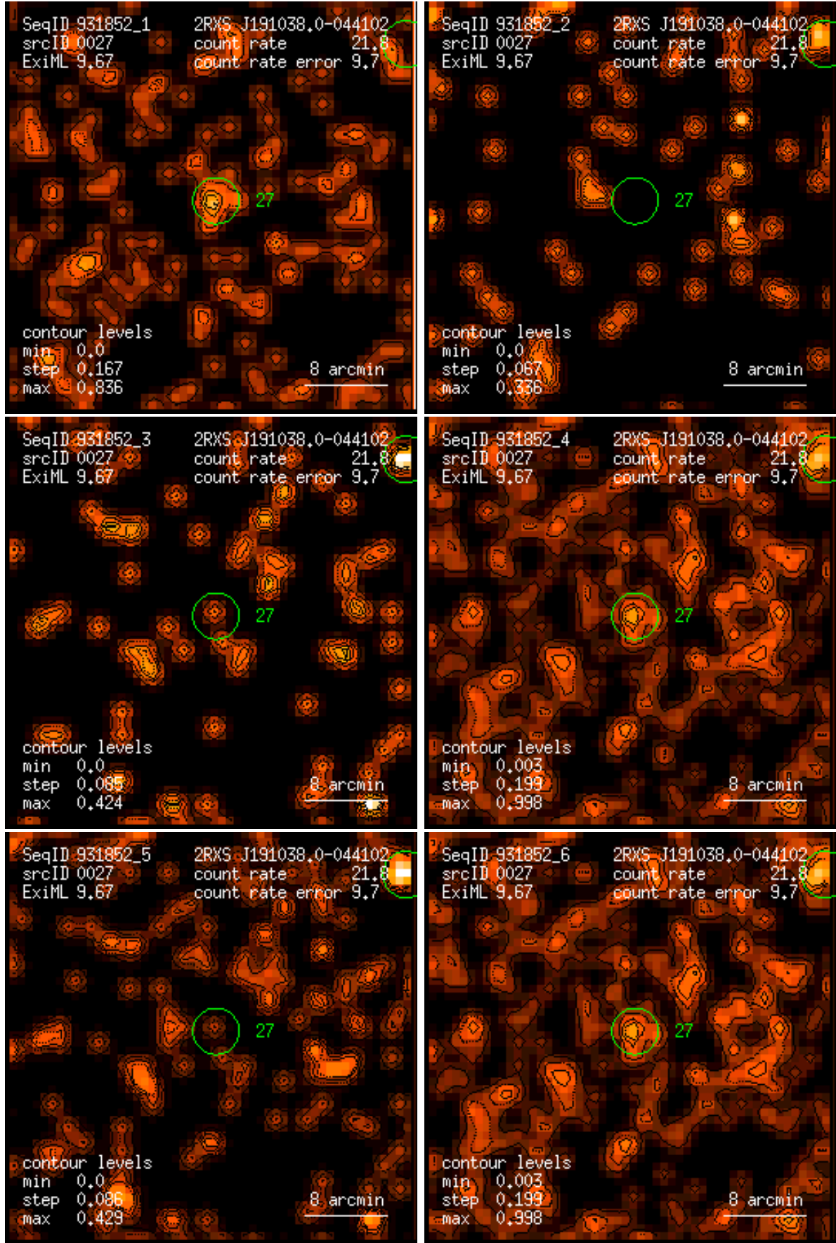
Figure 27: RASS 931852: detection 0027: band rate images, Gaussian filter: (1) PSPC channels 11 – 41, (2) 52 – 90, (3) 91 – 201, (4) 11 – 235, (5) 52 – 201, (6) 11 – 201. Broad band rates in counts/ks. Band rate contour levels in counts/ks/arcmin 2 .
