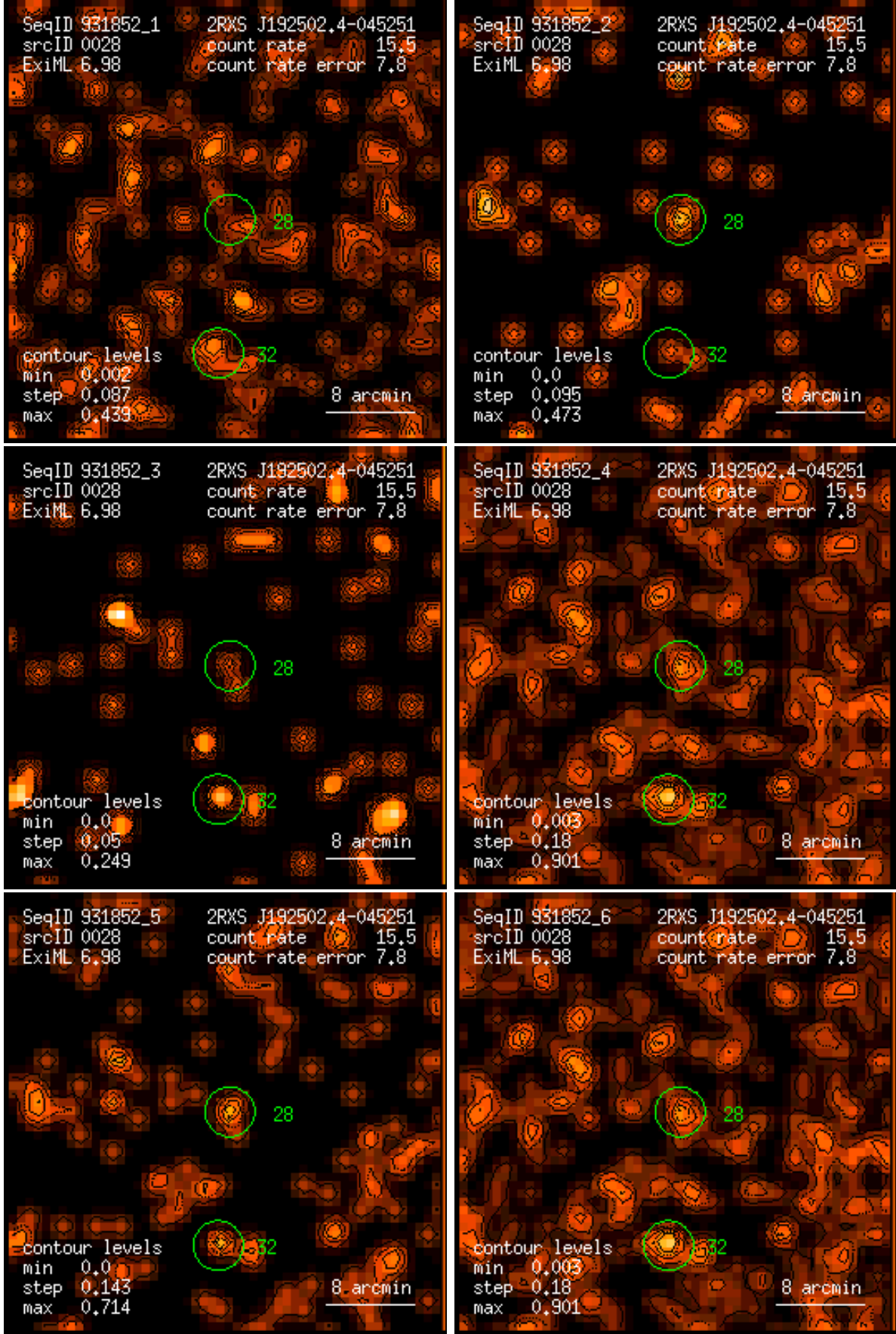
Figure 28: RASS 931852: detection 0028: band rate images, Gaussian filter: (1) PSPC channels 11 – 41, (2) 52 – 90, (3) 91 – 201, (4) 11 – 235, (5) 52 – 201, (6) 11 – 201. Broad band rates in counts/ks. Band rate contour levels in counts/ks/arcmin 2 .
