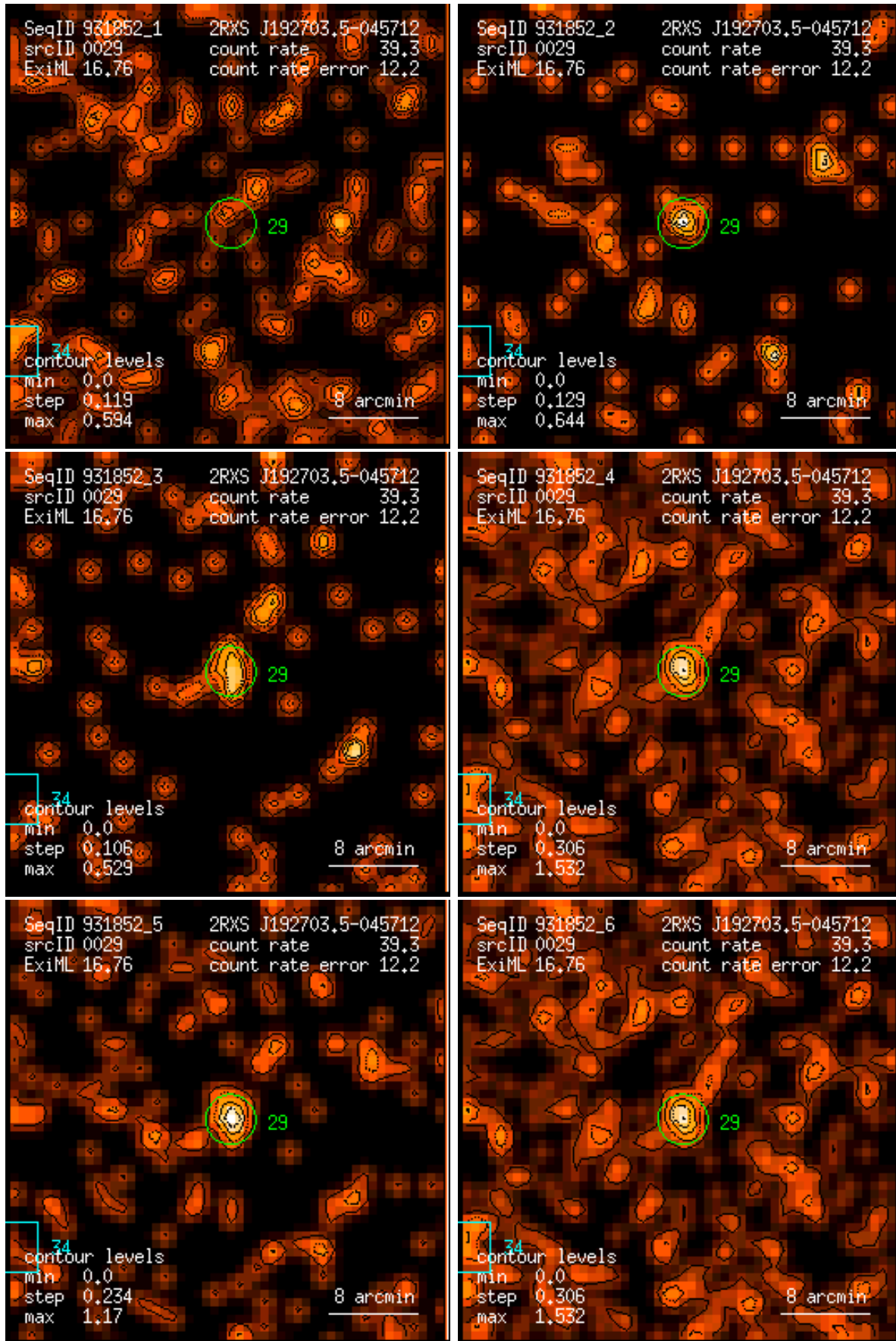
Figure 29: RASS 931852: detection 0029: band rate images, Gaussian filter: (1) PSPC channels 11 – 41, (2) 52 – 90, (3) 91 – 201, (4) 11 – 235, (5) 52 – 201, (6) 11 – 201. Broad band rates in counts/ks. Band rate contour levels in counts/ks/arcmin 2 .
