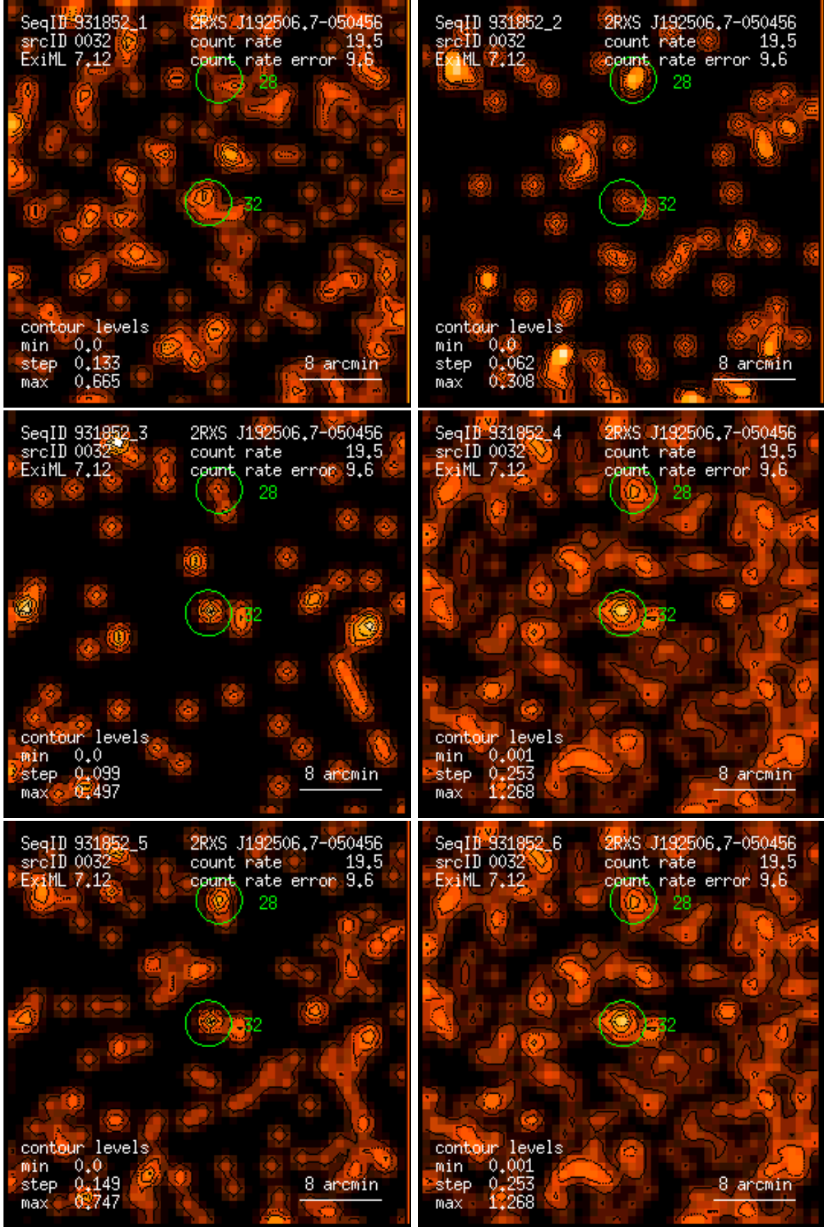
Figure 32: RASS 931852: detection 0032: band rate images, Gaussian filter: (1) PSPC channels 11 – 41, (2) 52 – 90, (3) 91 – 201, (4) 11 – 235, (5) 52 – 201, (6) 11 – 201. Broad band rates in counts/ks. Band rate contour levels in counts/ks/arcmin 2 .
