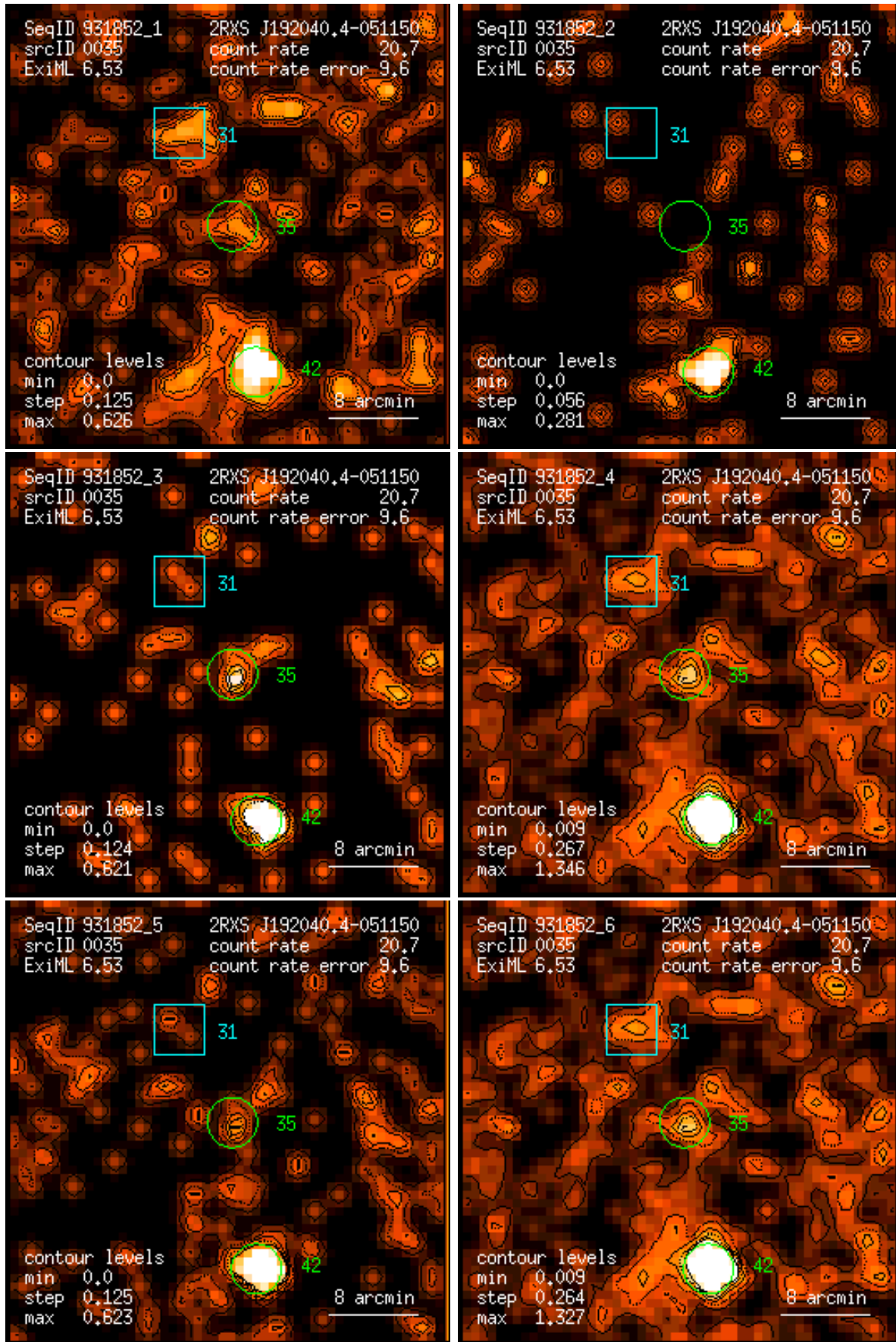
Figure 35: RASS 931852: detection 0035: band rate images, Gaussian filter: (1) PSPC channels 11 – 41, (2) 52 – 90, (3) 91 – 201, (4) 11 – 235, (5) 52 – 201, (6) 11 – 201. Broad band rates in counts/ks. Band rate contour levels in counts/ks/arcmin 2 .
