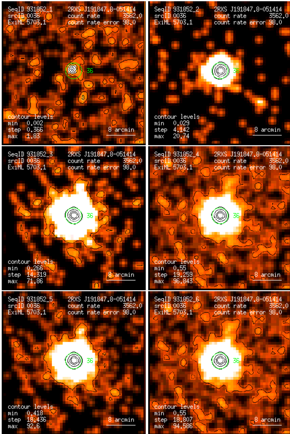
Figure 36: RASS 931852: detection 0036: band rate images, Gaussian filter: (1) PSPC channels 11 – 41, (2) 52 – 90, (3) 91 – 201, (4) 11 – 235, (5) 52 – 201, (6) 11 – 201. Broad band rates in counts/ks. Band rate contour levels in counts/ks/arcmin 2 .
