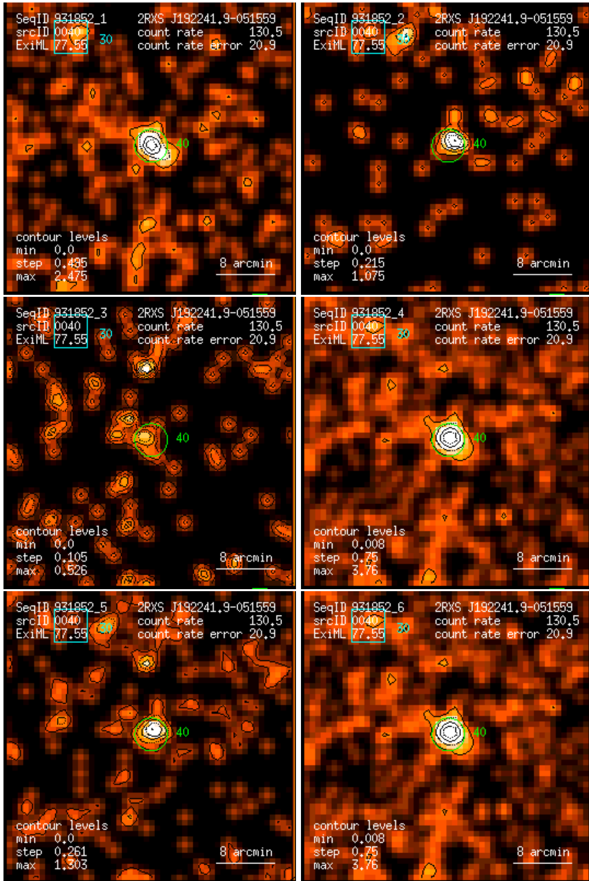
Figure 40: RASS 931852: detection 0040: band rate images, Gaussian filter: (1) PSPC channels 11 – 41, (2) 52 – 90, (3) 91 – 201, (4) 11 – 235, (5) 52 – 201, (6) 11 – 201. Broad band rates in counts/ks. Band rate contour levels in counts/ks/arcmin 2 .
