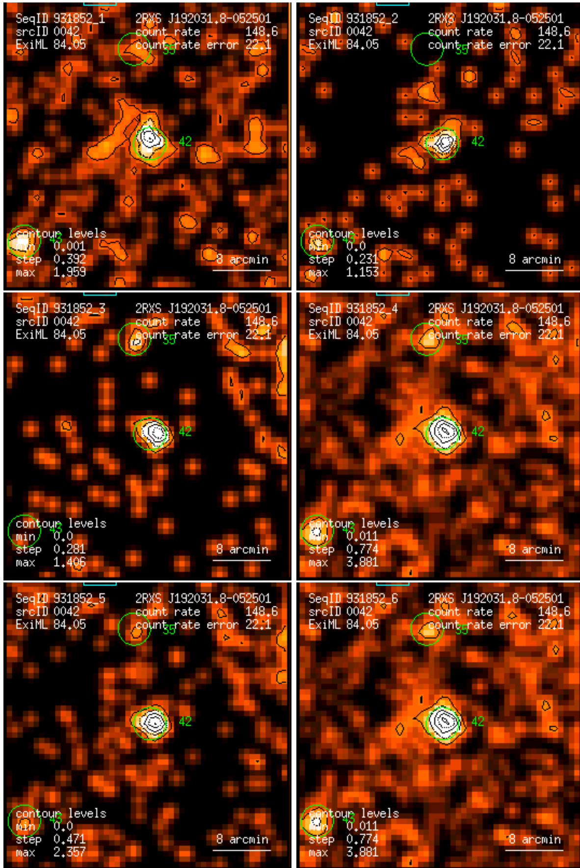
Figure 42: RASS 931852: detection 0042: band rate images, Gaussian filter: (1) PSPC channels 11 – 41, (2) 52 – 90, (3) 91 – 201, (4) 11 – 235, (5) 52 – 201, (6) 11 – 201. Broad band rates in counts/ks. Band rate contour levels in counts/ks/arcmin 2 .
