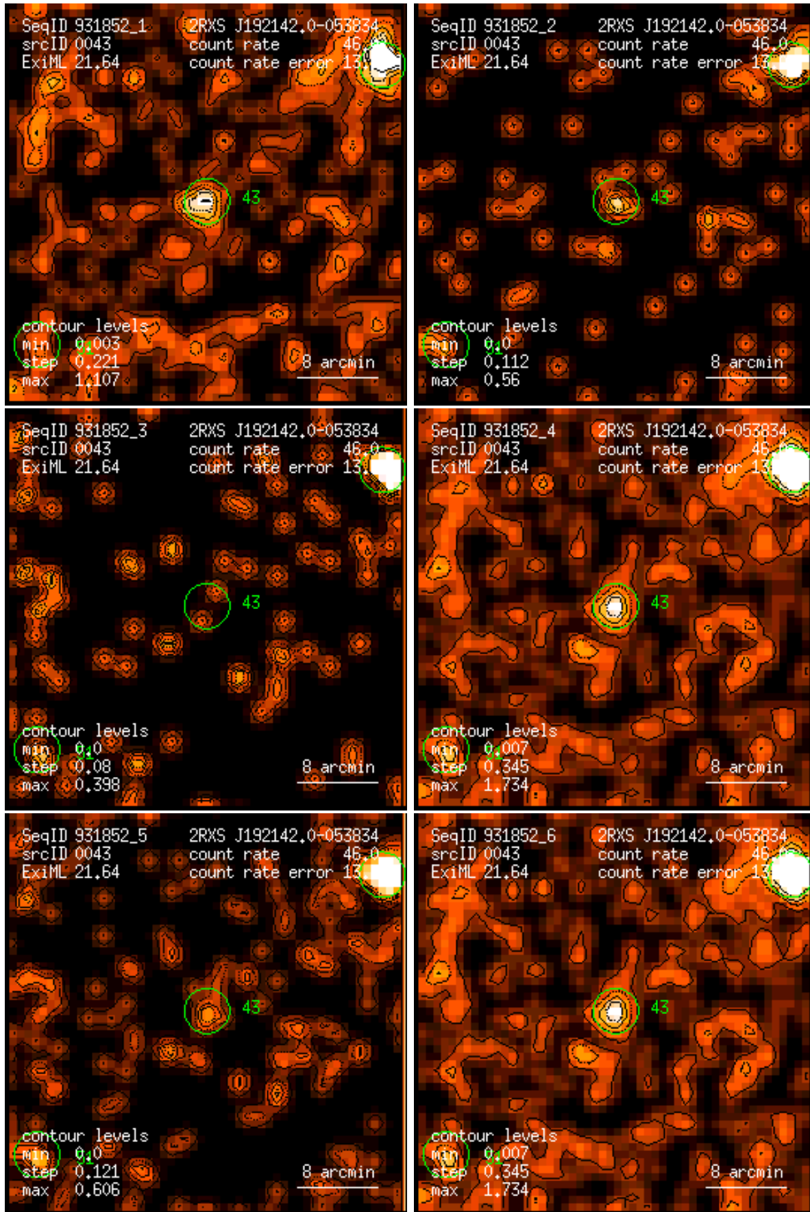
Figure 43: RASS 931852: detection 0043: band rate images, Gaussian filter: (1) PSPC channels 11 – 41, (2) 52 – 90, (3) 91 – 201, (4) 11 – 235, (5) 52 – 201, (6) 11 – 201. Broad band rates in counts/ks. Band rate contour levels in counts/ks/arcmin 2 .
