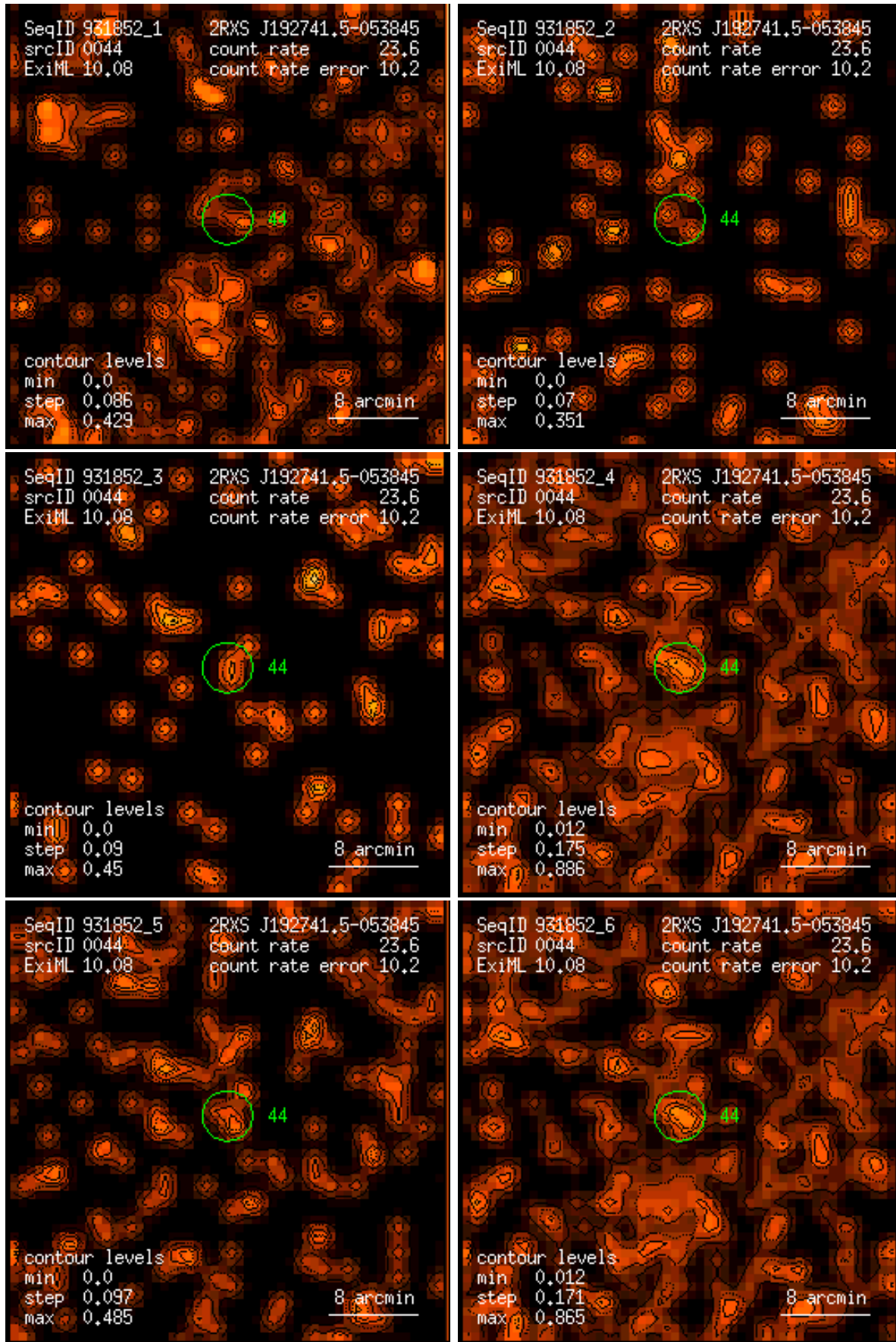
Figure 44: RASS 931852: detection 0044: band rate images, Gaussian filter: (1) PSPC channels 11 – 41, (2) 52 – 90, (3) 91 – 201, (4) 11 – 235, (5) 52 – 201, (6) 11 – 201. Broad band rates in counts/ks. Band rate contour levels in counts/ks/arcmin 2 .
