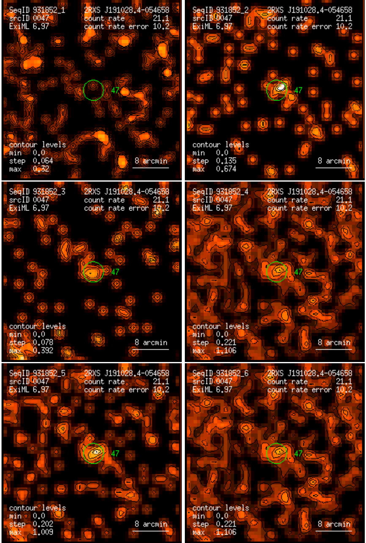
Figure 47: RASS 931852: detection 0047: band rate images, Gaussian filter: (1) PSPC channels 11 – 41, (2) 52 – 90, (3) 91 – 201, (4) 11 – 235, (5) 52 – 201, (6) 11 – 201. Broad band rates in counts/ks. Band rate contour levels in counts/ks/arcmin 2 .
