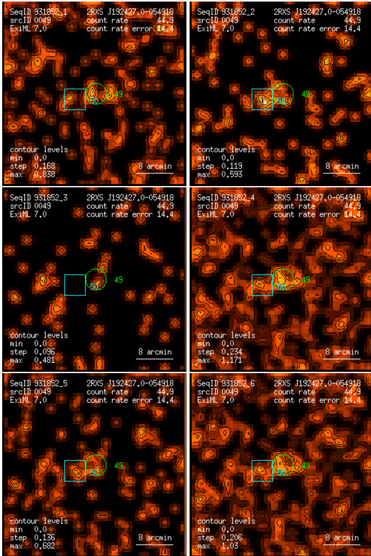
Figure 49: RASS 931852: detection 0049: band rate images, Gaussian filter: (1) PSPC channels 11 – 41, (2) 52 – 90, (3) 91 – 201, (4) 11 – 235, (5) 52 – 201, (6) 11 – 201. Broad band rates in counts/ks. Band rate contour levels in counts/ks/arcmin 2 .
